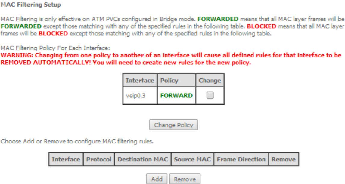
Figure 117: Advanced Setup, Security – MAC filtering Setup window –Change policy
