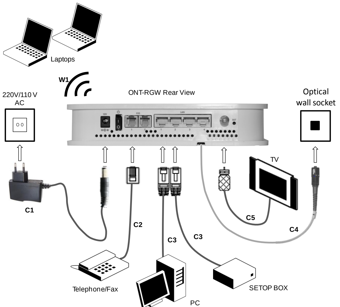
Figure 19: ONT-RGW connections
