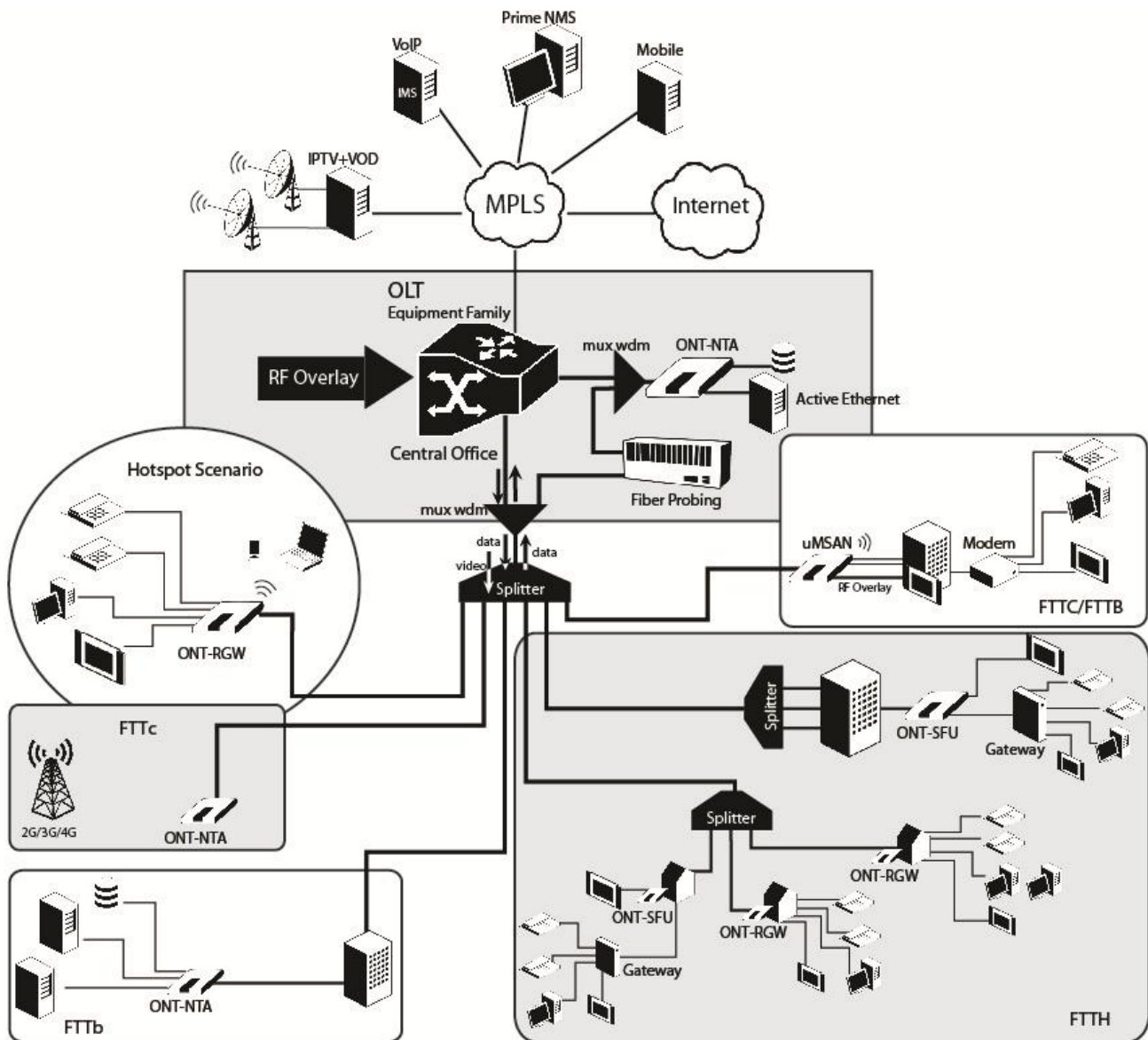
Figure 1: ONT-RGW applications scenario
