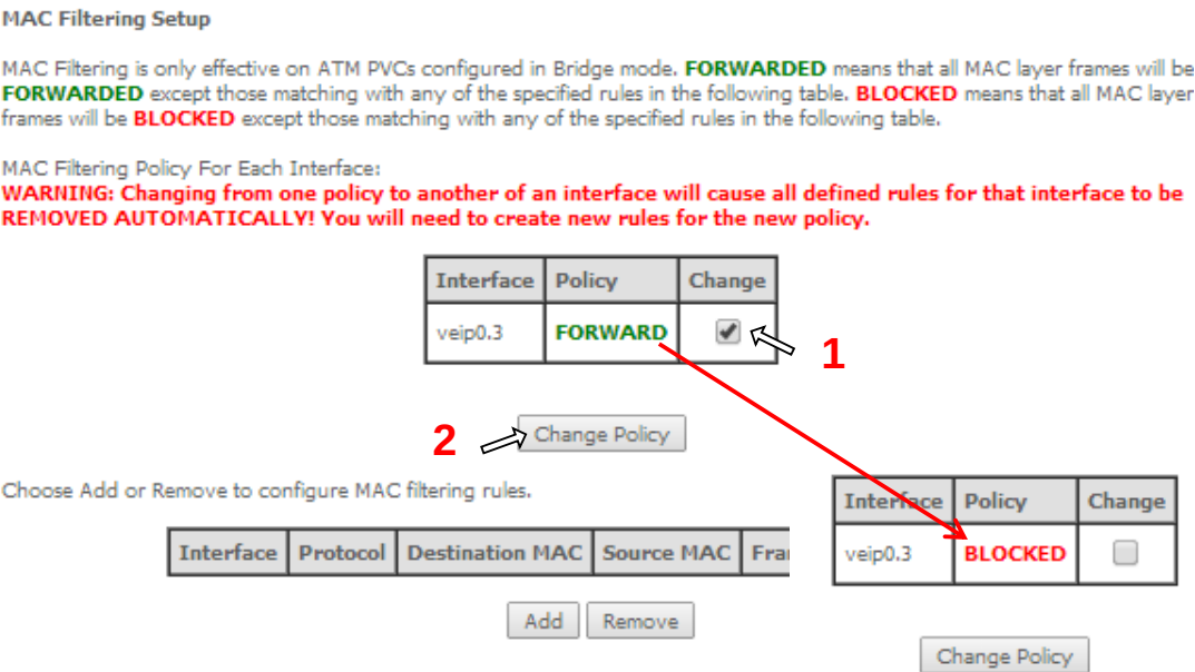
Figure 117: Advanced Setup, Security – MAC filtering Setup window –Change policy
