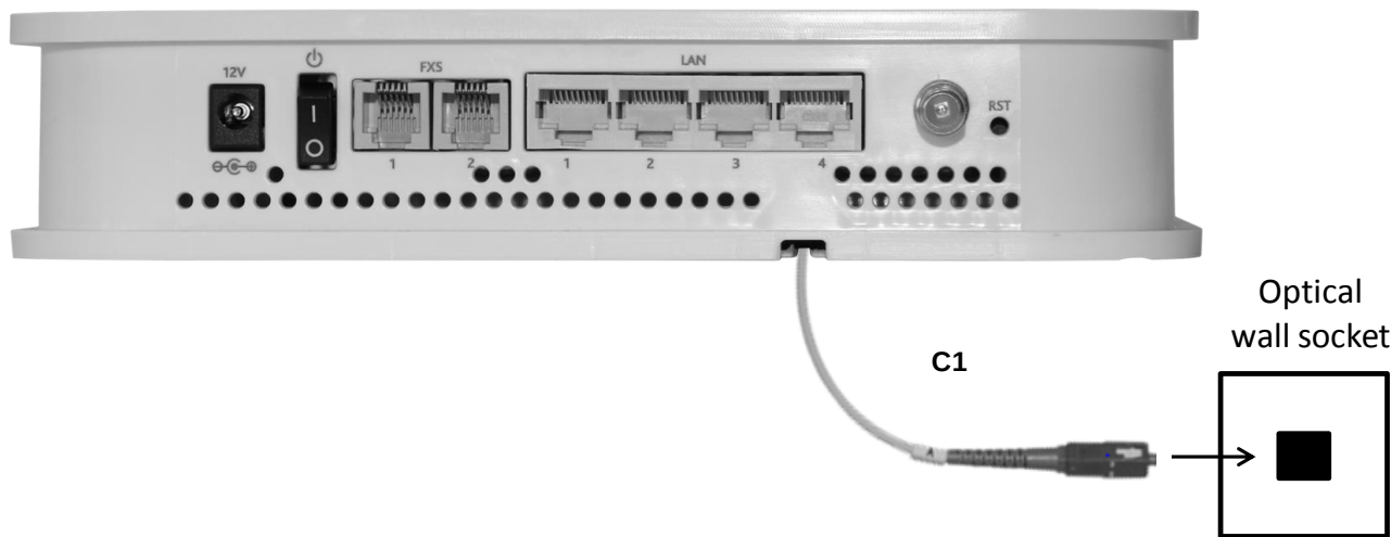
Figure 18: Interfaces connection 1 (PON Interface)
