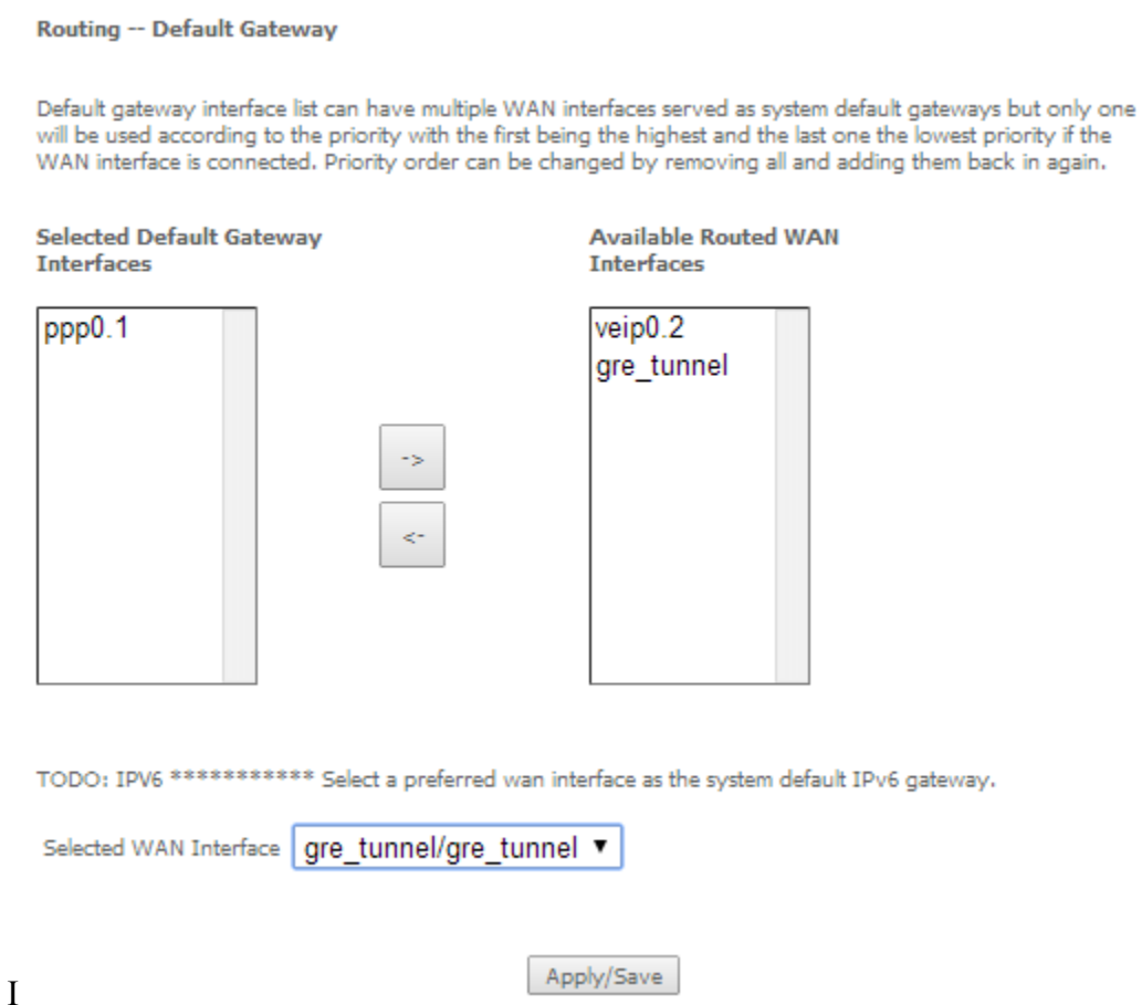
Figure 138: Advanced Setup, Routing-Default Gateway Configuration window
