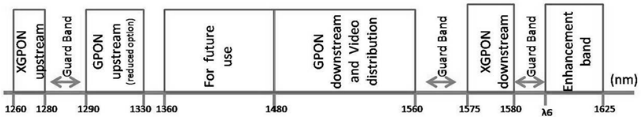
Figure 13: Wavelength planning
