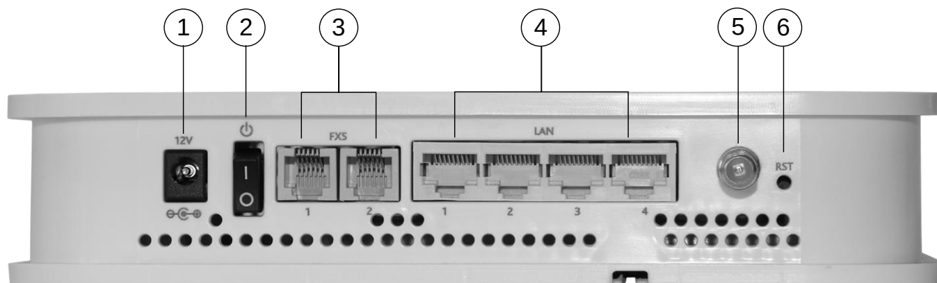
Figure 15: ONT-RGW connections 1
