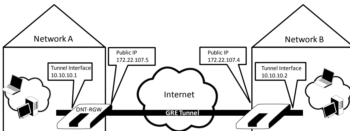
Figure 72: GRE Tunnel configuration example ate the Network A ONT-RGW
