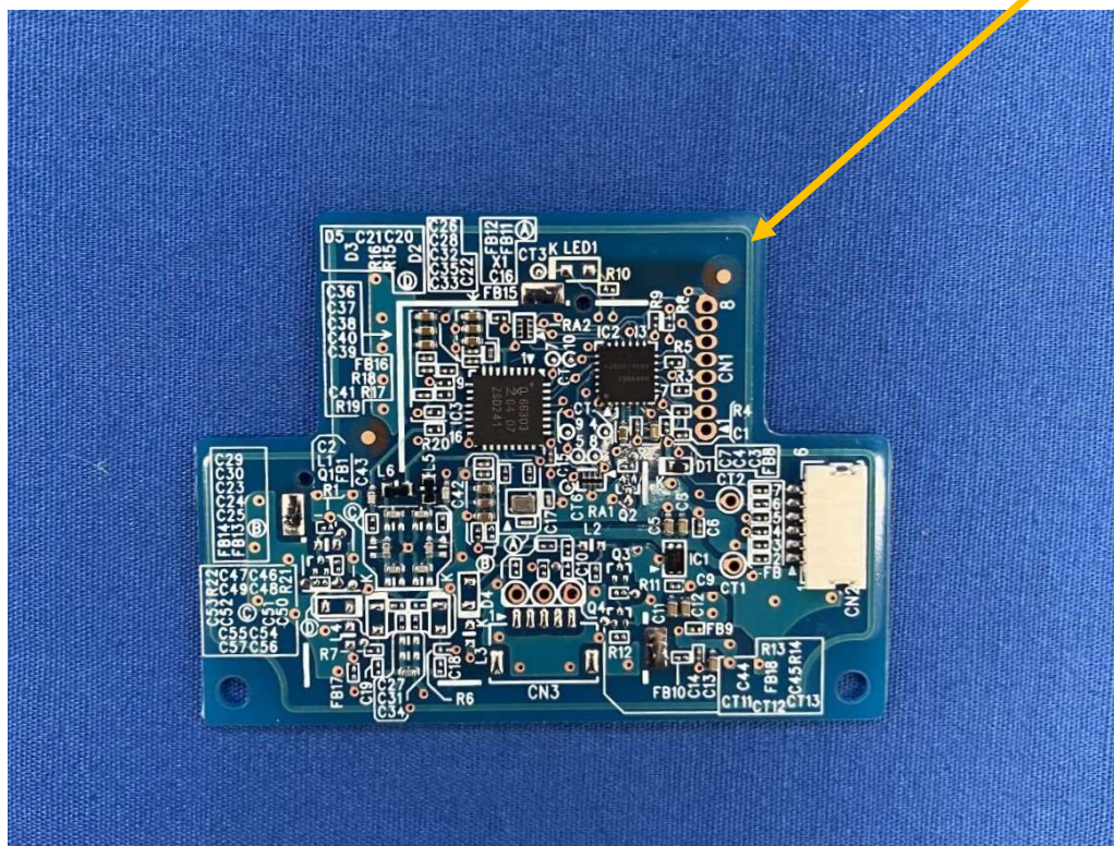
Component side wo shield
