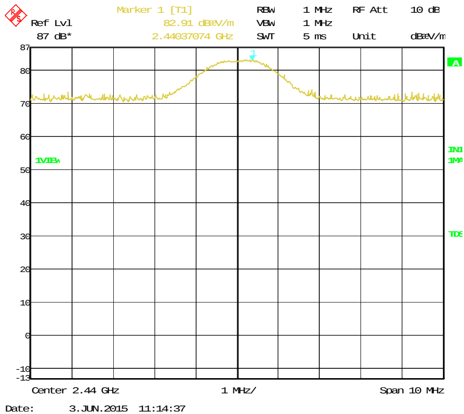
Figure 25 2440.0 MHz – Horizontal
