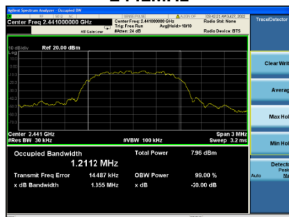
2441MHz
