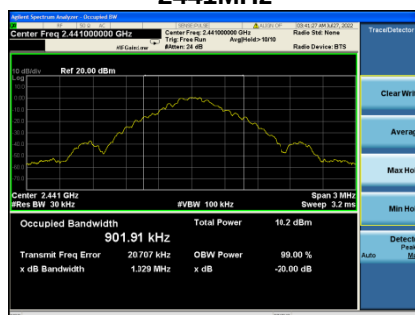
2441MHz
