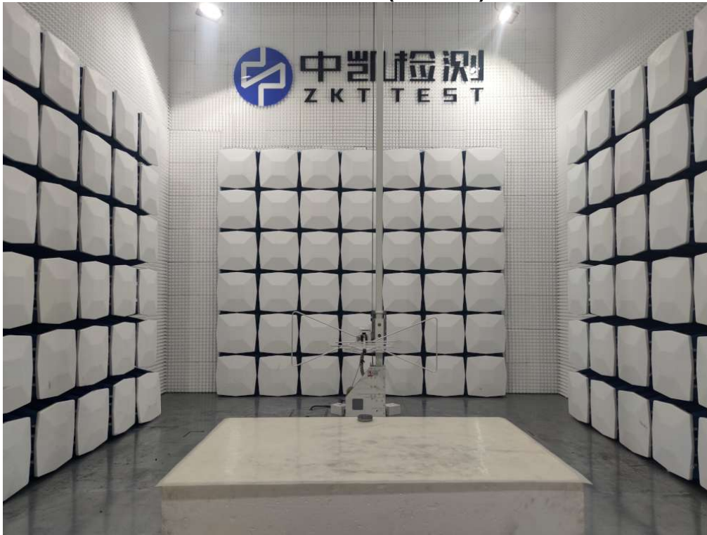
RadiatedEmission(Below 1G)
