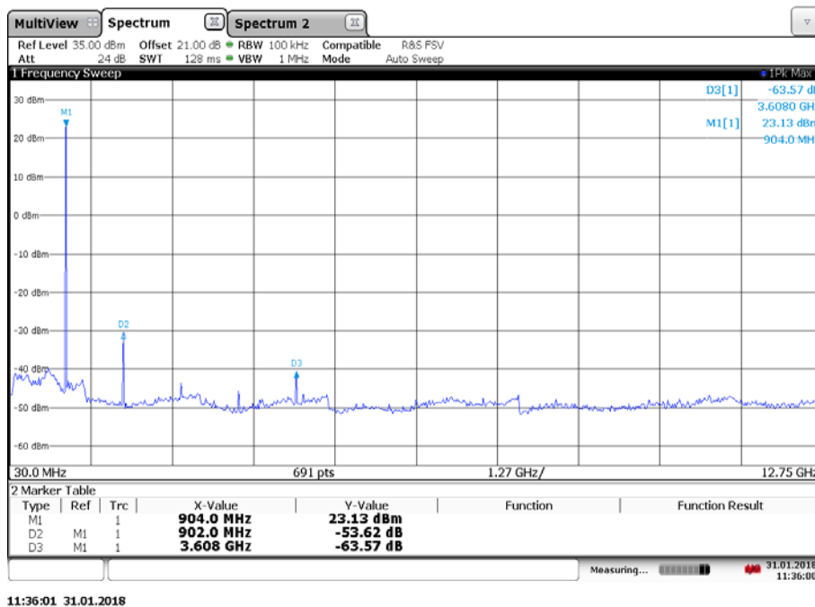
Plot 4: Middle channel, 30 MHz – 12.75 GHz
