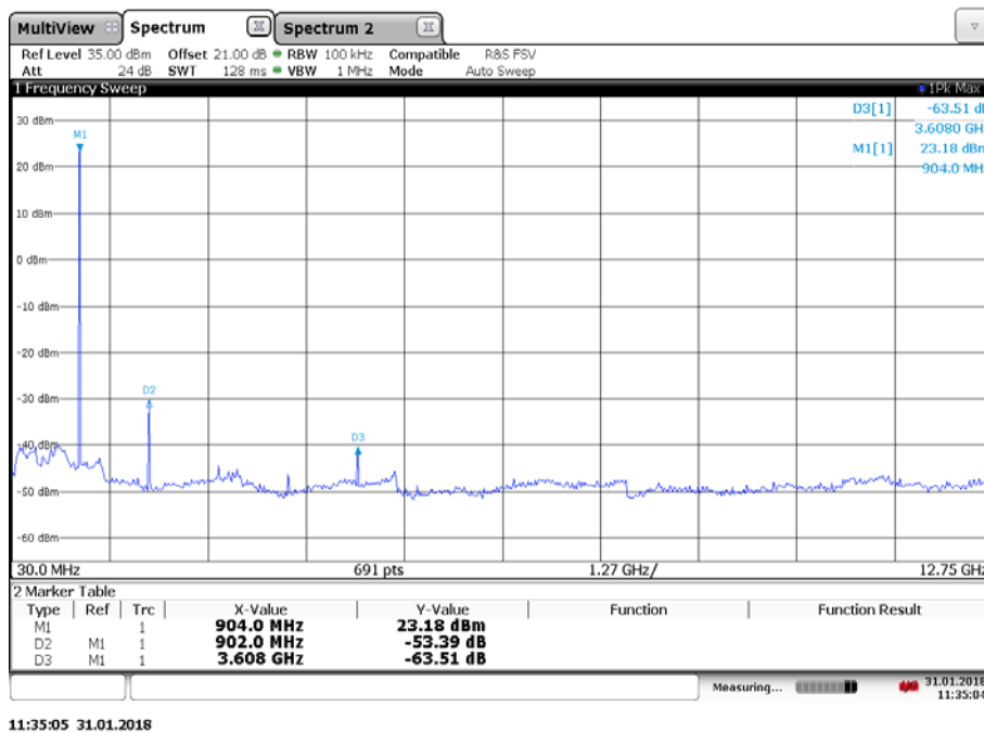
Plot 2: Low channel, 30 MHz – 12.75 GHz
