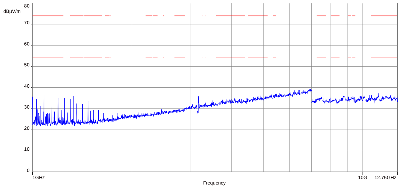
Plot 4: 1GHz – 12.75 GHz, RX-Mode, horizontal &amp; vertical polarisation (valid for all channels)
