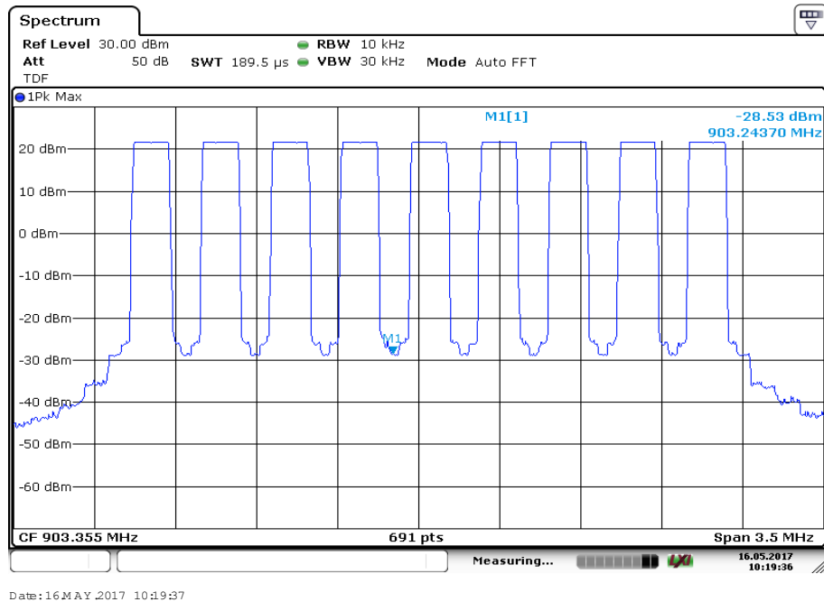
Plot 1: Number of macro channels (9)
