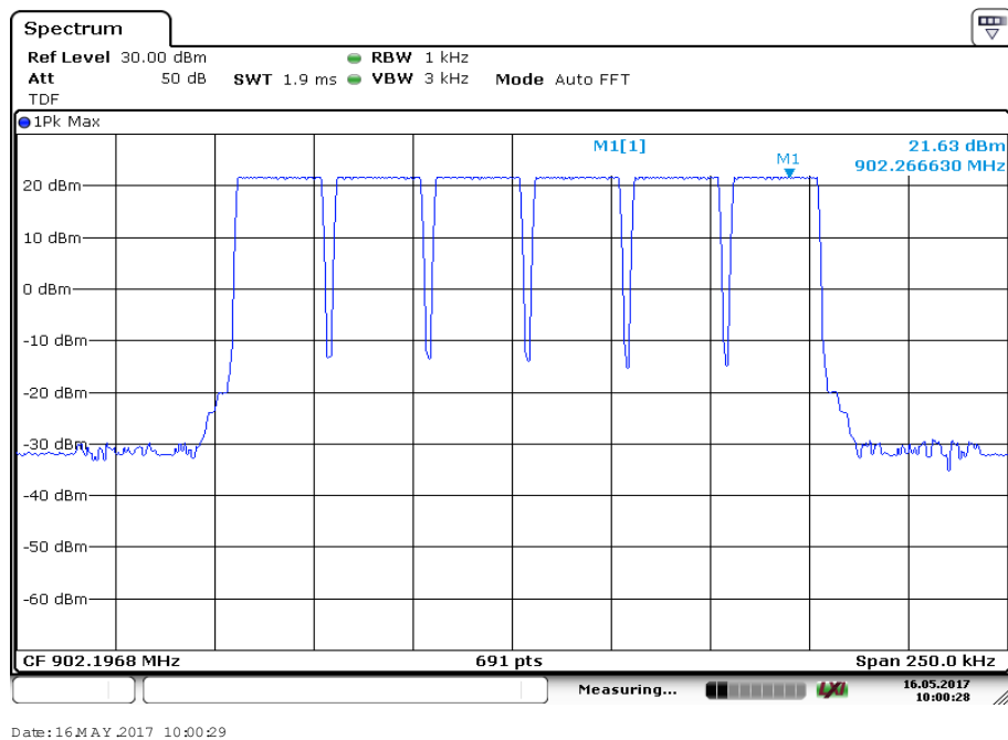
Plot 2: Number of micro channels in one single macro channel zoomed (6)
