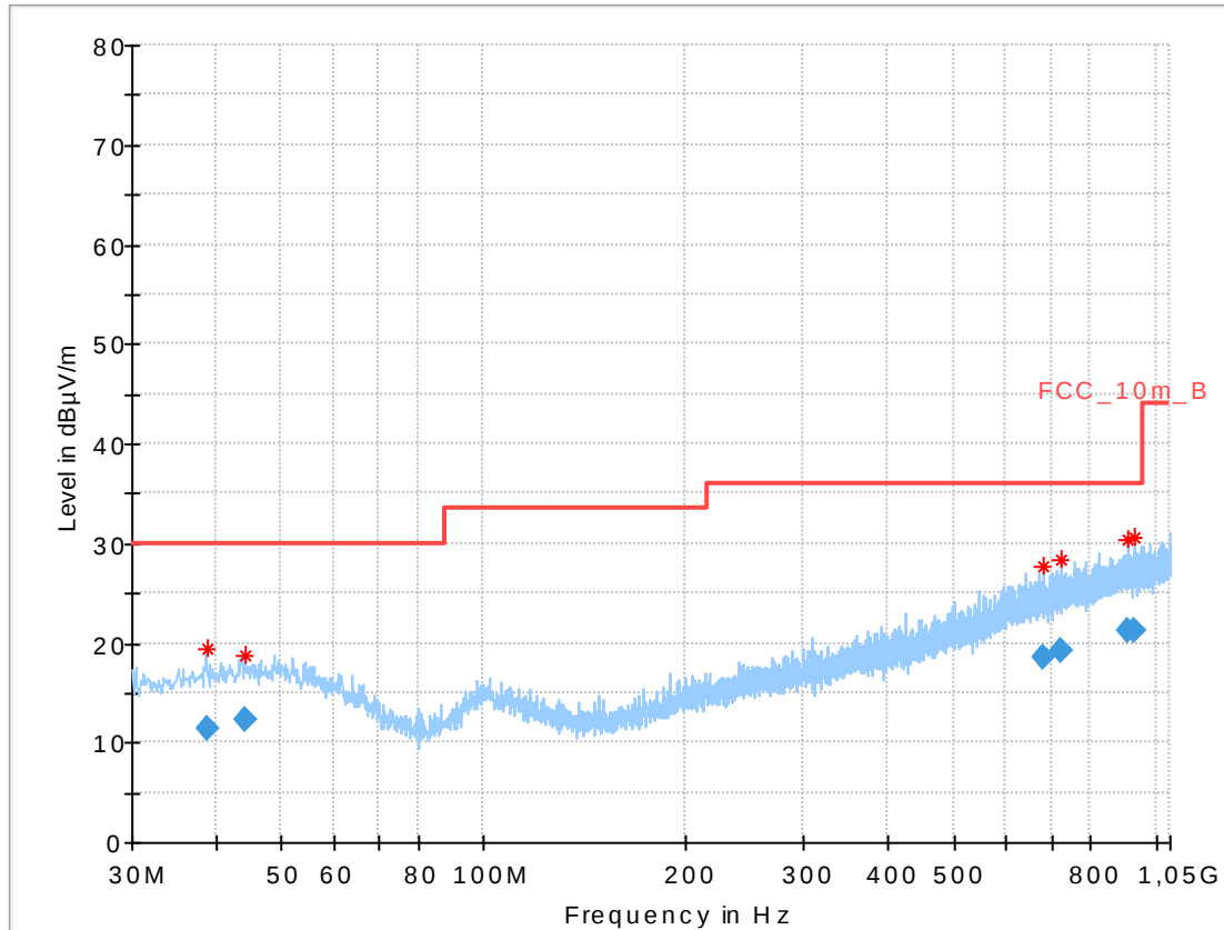
Plot 4: 30 MHz – 1 GHz, horizontal &amp; vertical polarisation (RX-Mode)
