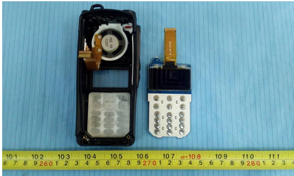
EUT –Cover off View 3
