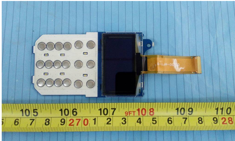
EUT – Key & LCD Board Top View
