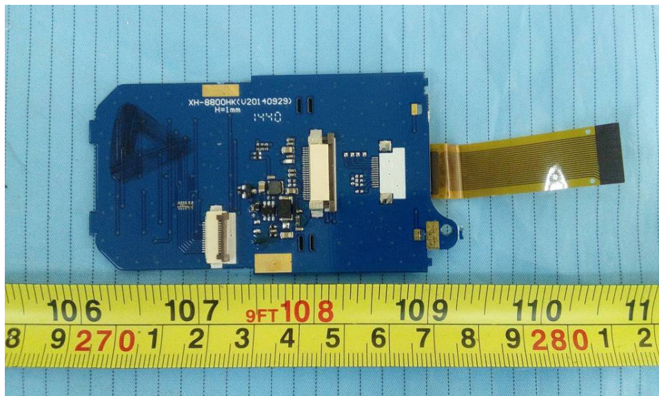
EUT – Key & LCD Board Bottom View
