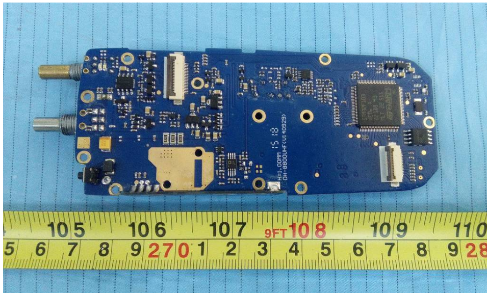
EUT – Main Board Bottom View
