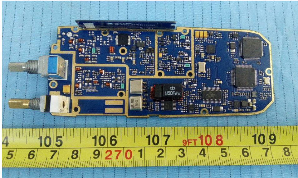
EUT – Main Board Top View
