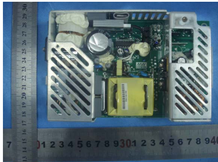
EUT – Power Supply Top View
