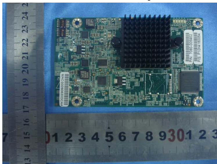
EUT - Circuit Board 2 Top View
