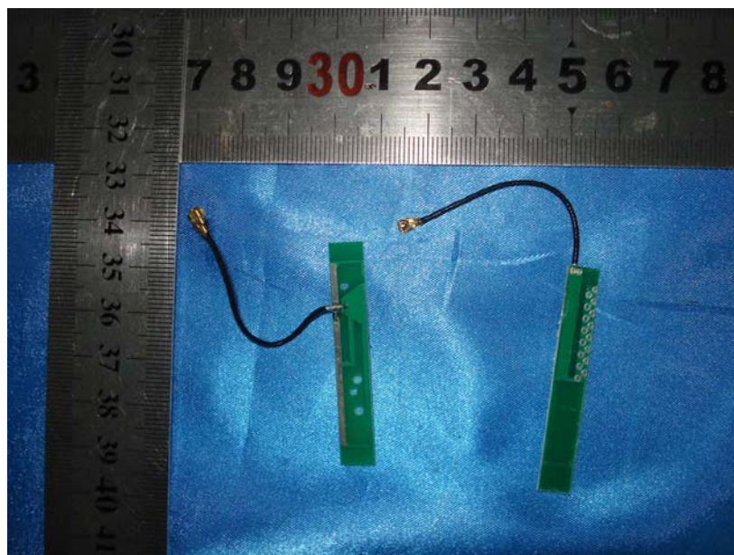
Antenna View
