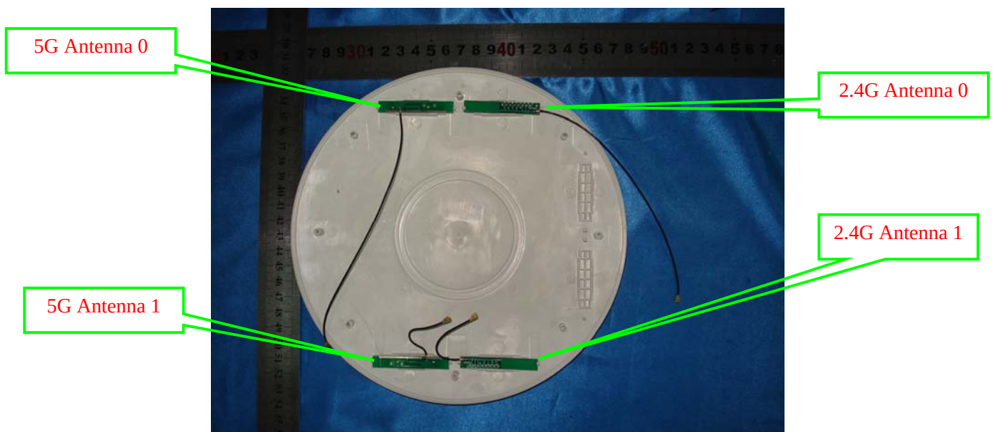
EUT – Cover off 2 View
