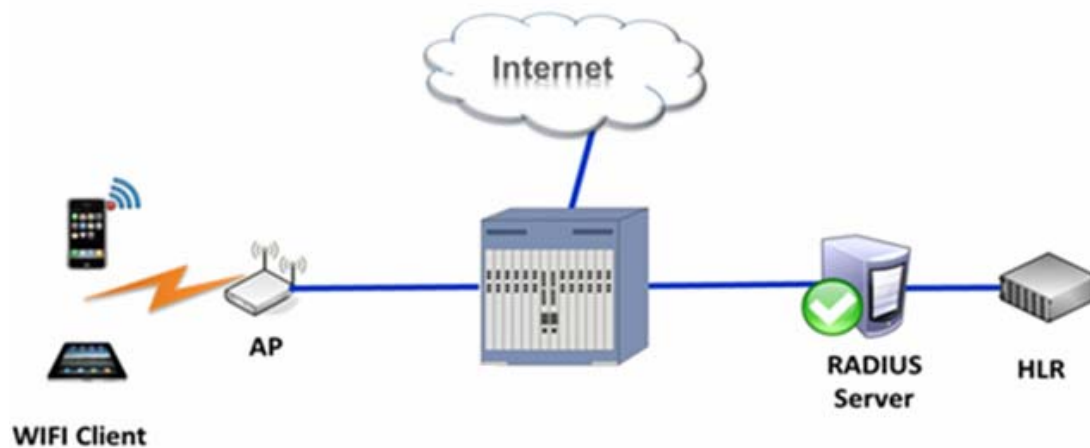
Figure 9-1 EAP-SIM authentication
