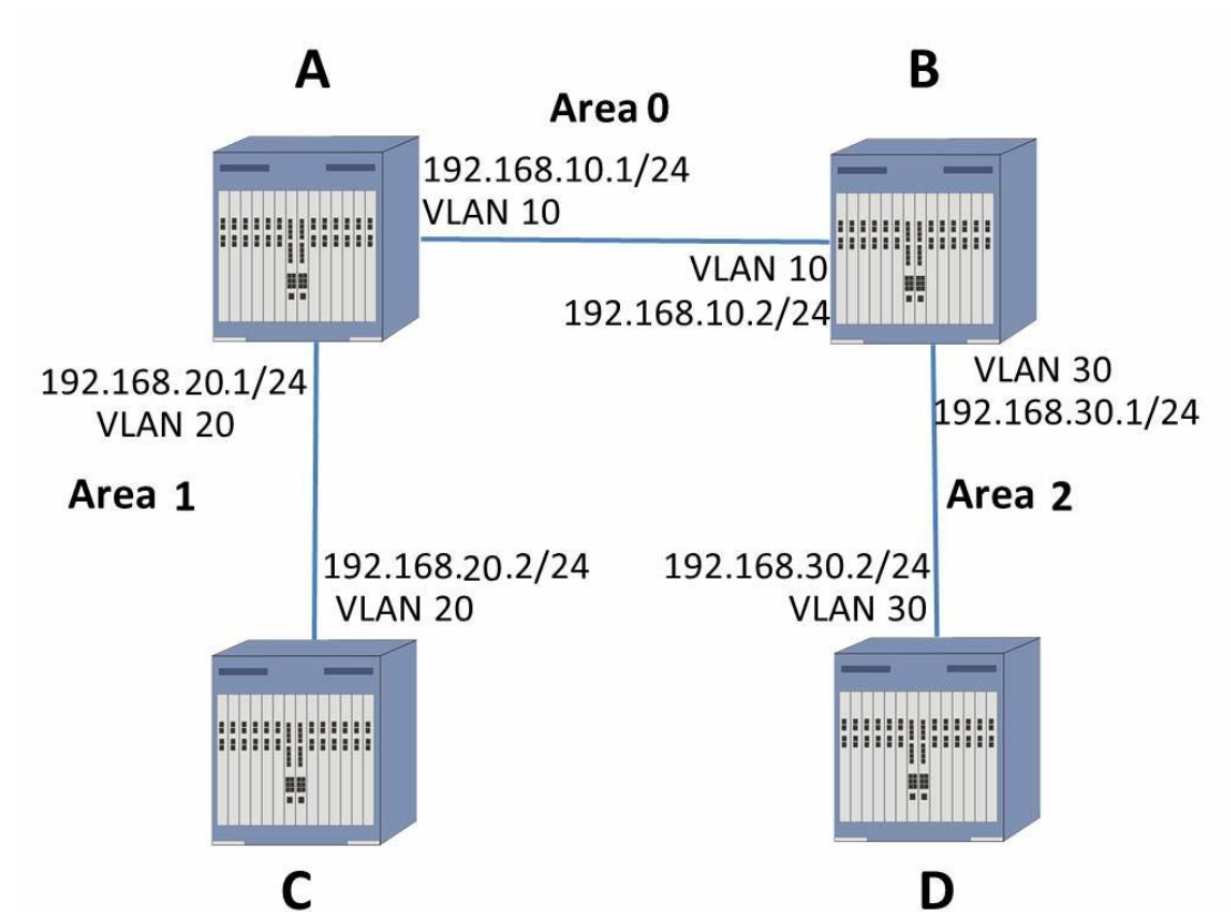
Figure 6-1 OSPF configuration example
