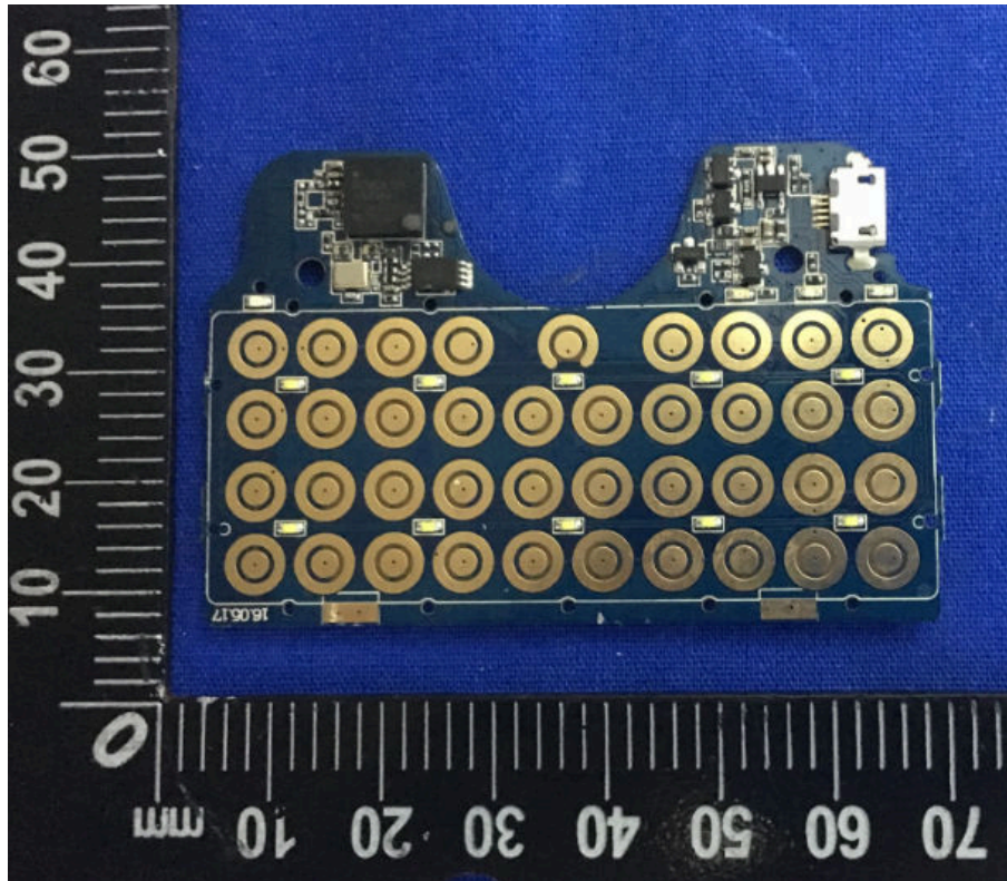
EUT – PCB View
