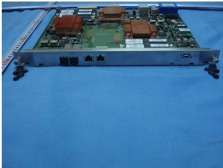
EUT – PCB2 Front View
