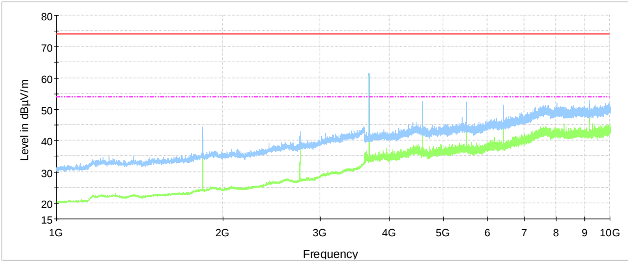
Figure 8.3-12: Cabinet Radiated spurious emissions 1 to 10 GHz, High channel
