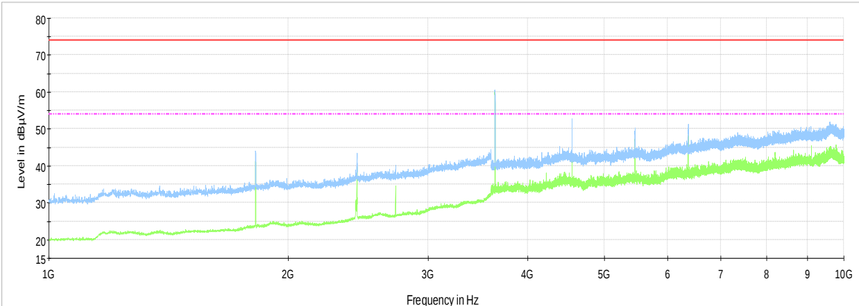
Figure 8.3-11: Cabinet Radiated spurious emissions 1 to 10 GHz, Low channel
