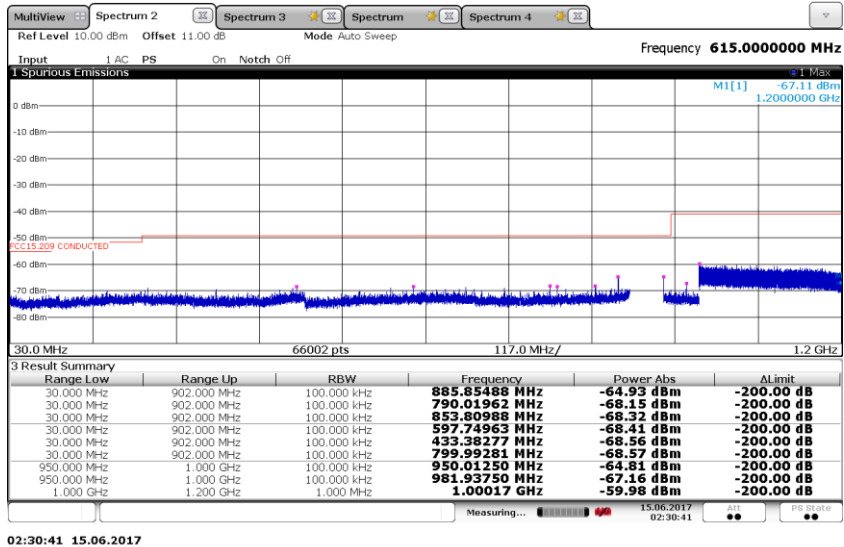
Figure 8.3-6: Conducted spurious emissions of restricted band 30 MHz to 1.2 GHz, High channel
