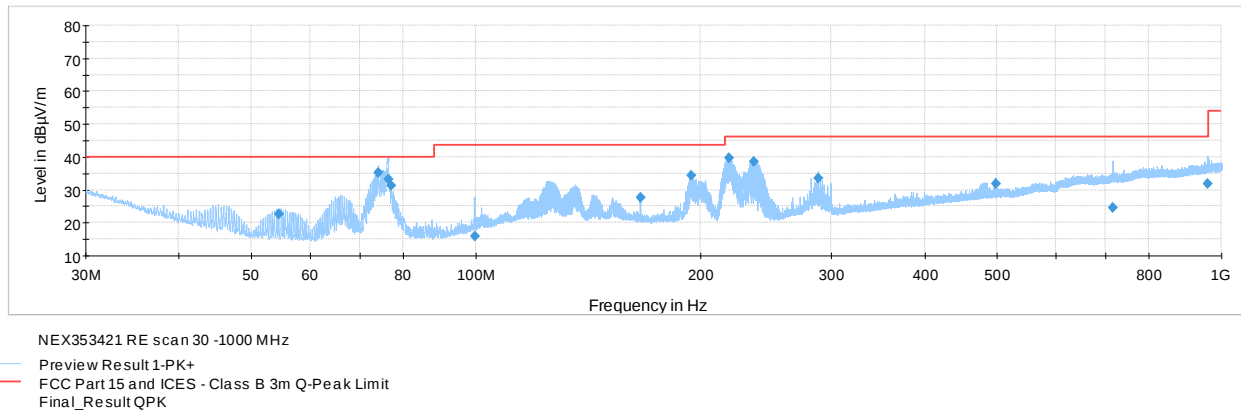
Figure 8.1-1: Radiated emissions spectral plot (30 to 1000 MHz)
