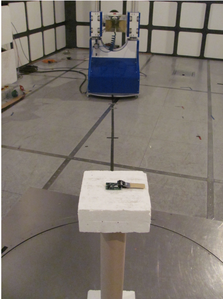
Radiated Emissions 1-10GHz
