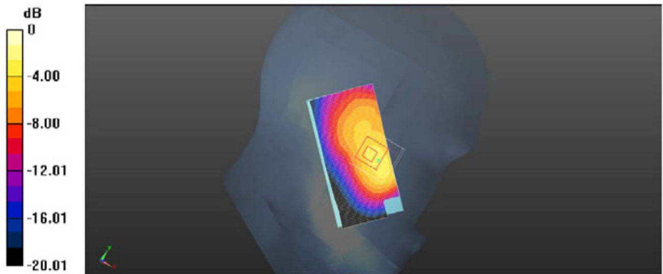
Plot 1: Left Head Tilt (GSM850 High Channel)
