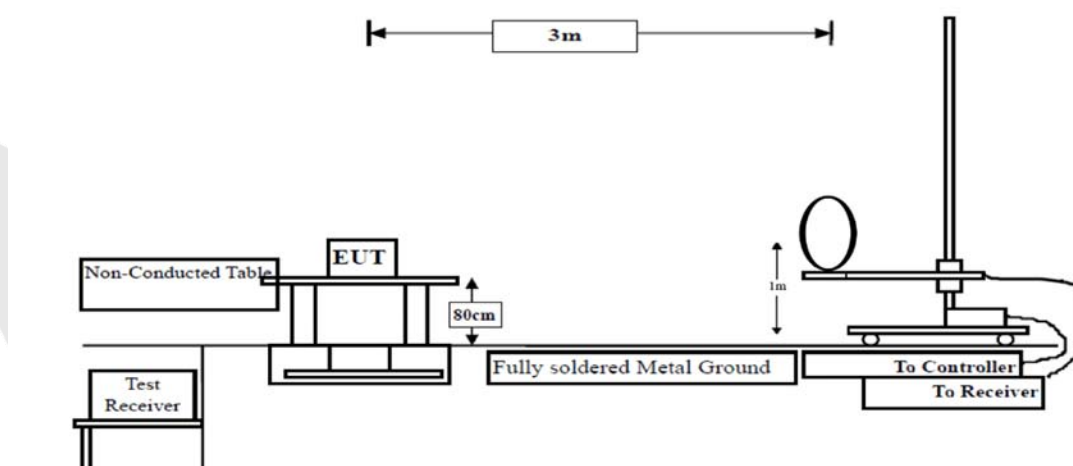
Figure 1. Below 30MHz
