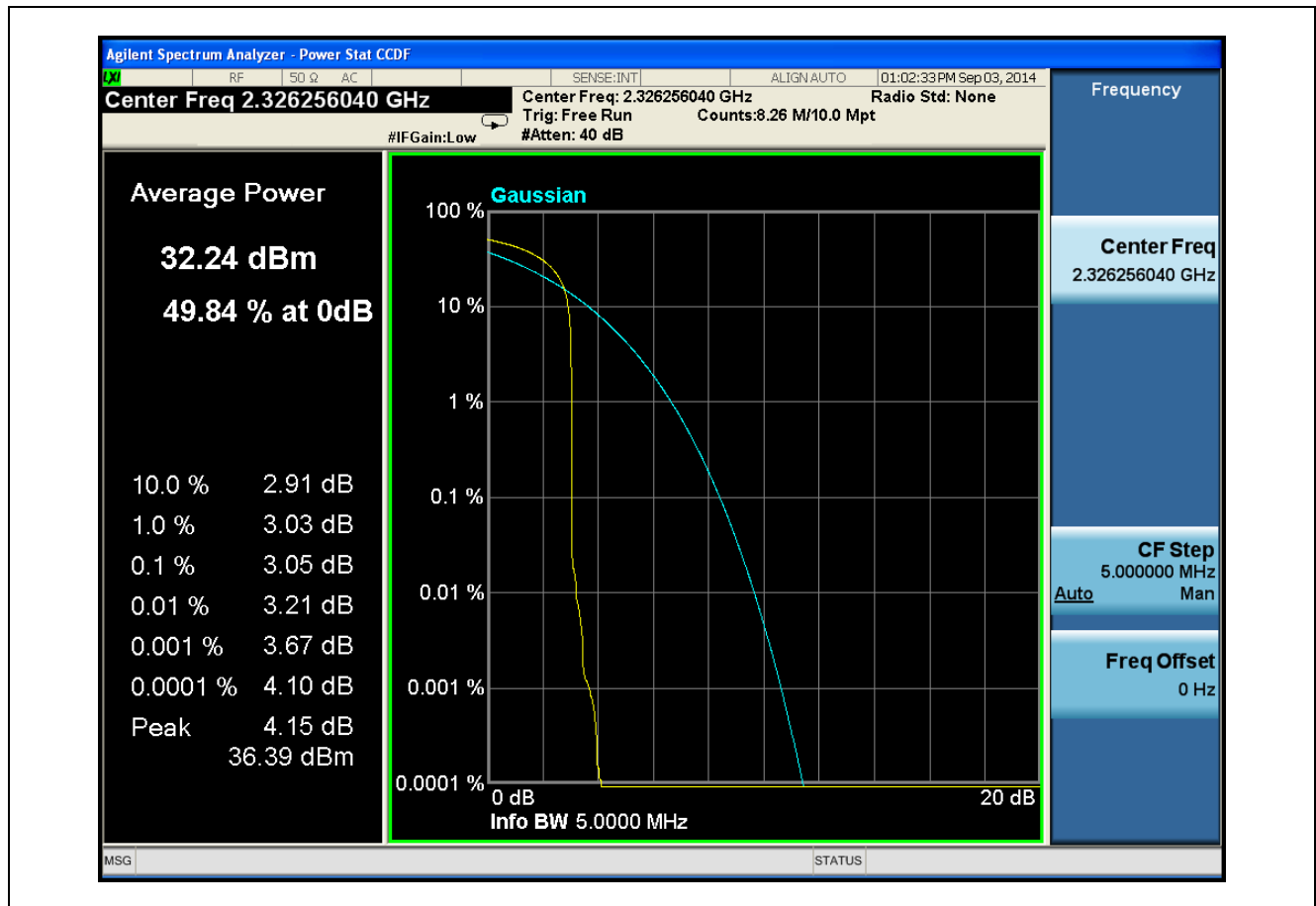
Plot 5.1.4.2.3. Peak-to-Average Power Ratio, LB Diversity, 2326.256040 MHz, OFDM Modulation, CCDF
