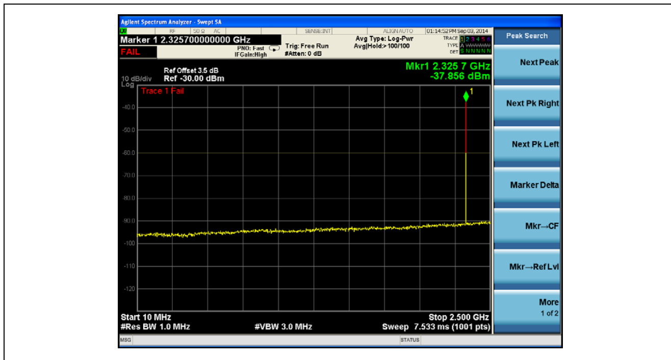
Plot 5.3.4.2.9. Conducted Spurious Emissions for LB Diversity, 2326.256040 MHz, 10 MHz – 2.5 GHz
