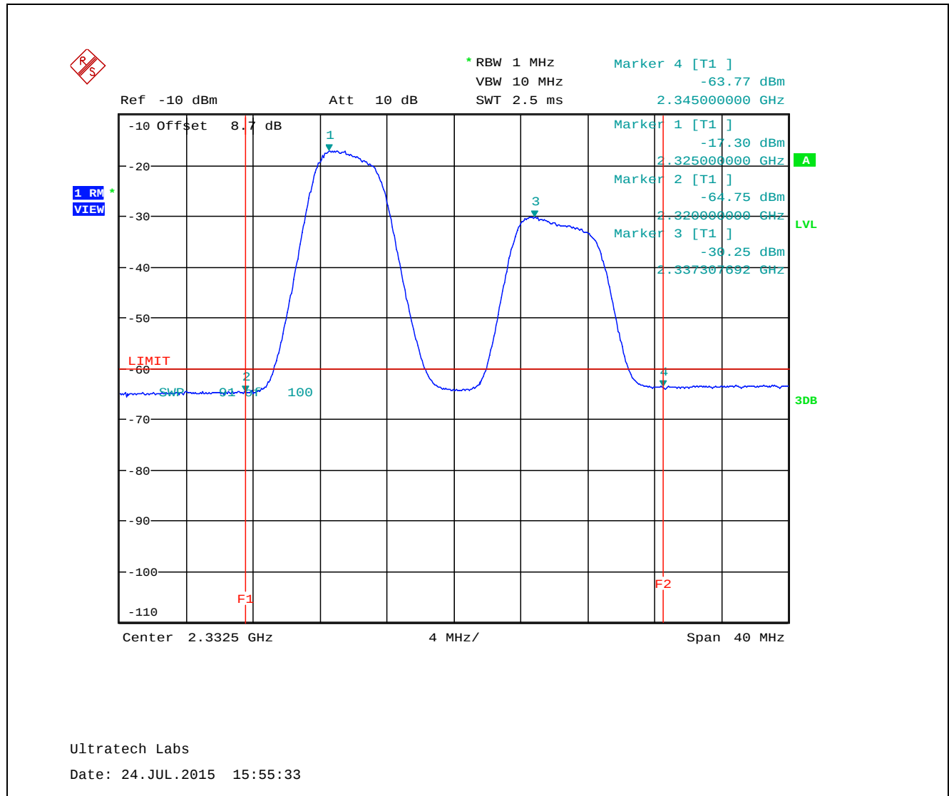
Plot 5.3.4.1.1. Band-Edge RF Conducted Emissions, Low & High Bands, OFDM Modulation, Average Detector
