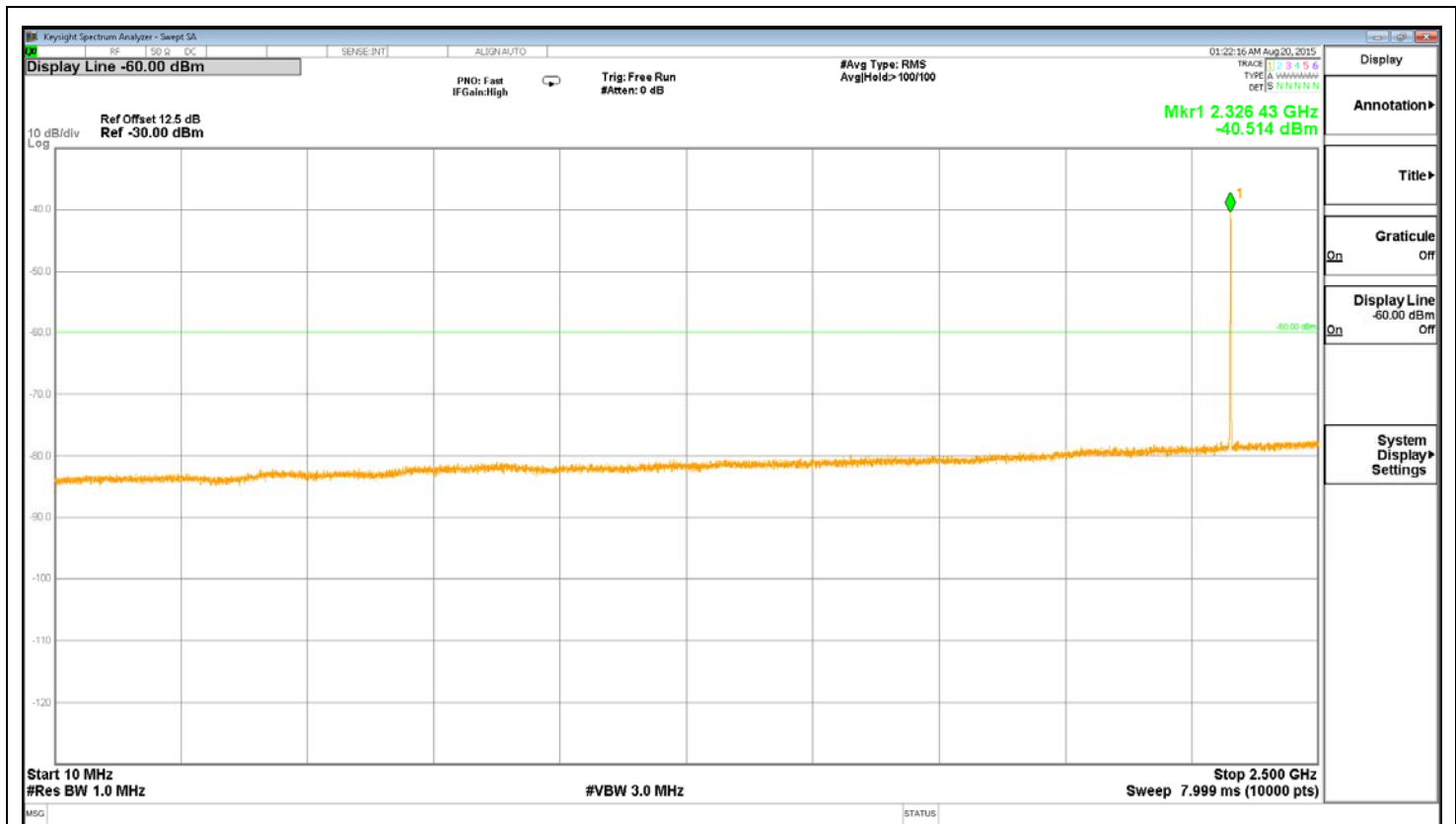
Plot 5.3.4.2.5. Conducted Spurious Emissions for LB Diversity, 2326.256040 MHz, 10 MHz – 2.5 GHz
