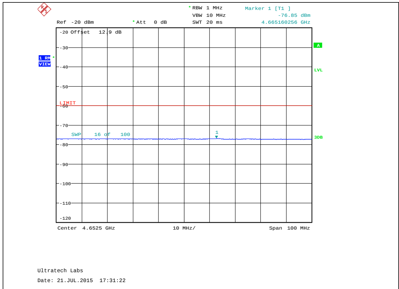
Plot 5.3.4.2.3. Conducted Spurious Emissions for LB + HB, Second Harmonic 4677.5 MHz Check with T-Splitter Connected
