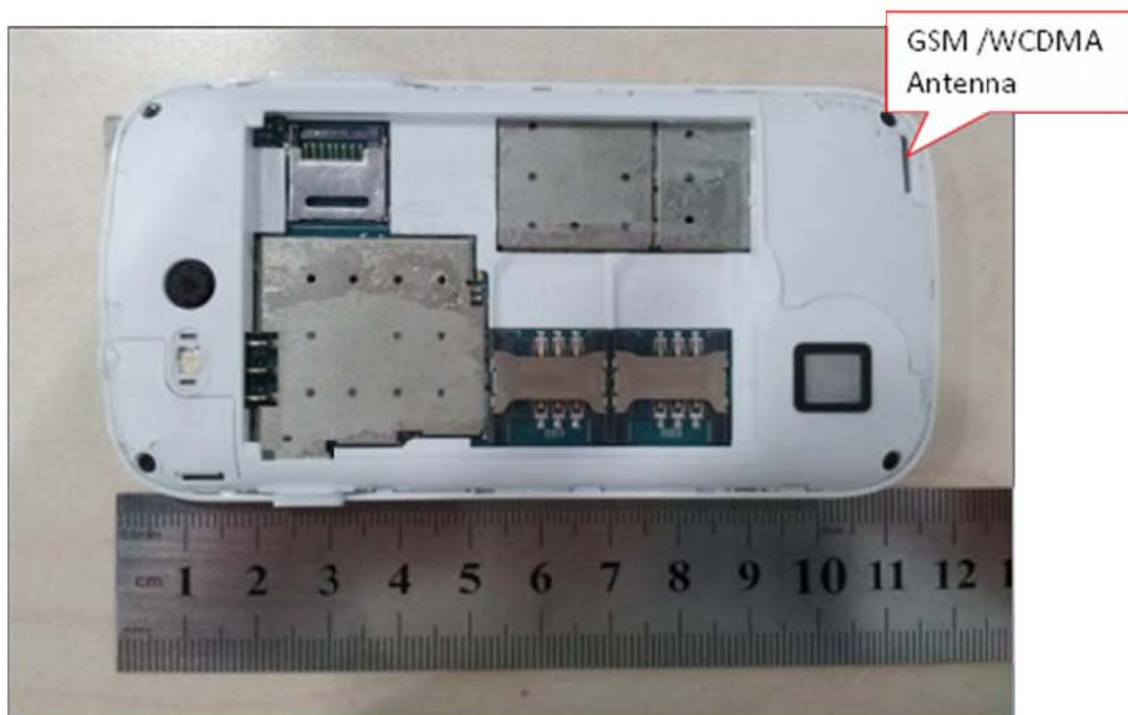
Antenna Location
