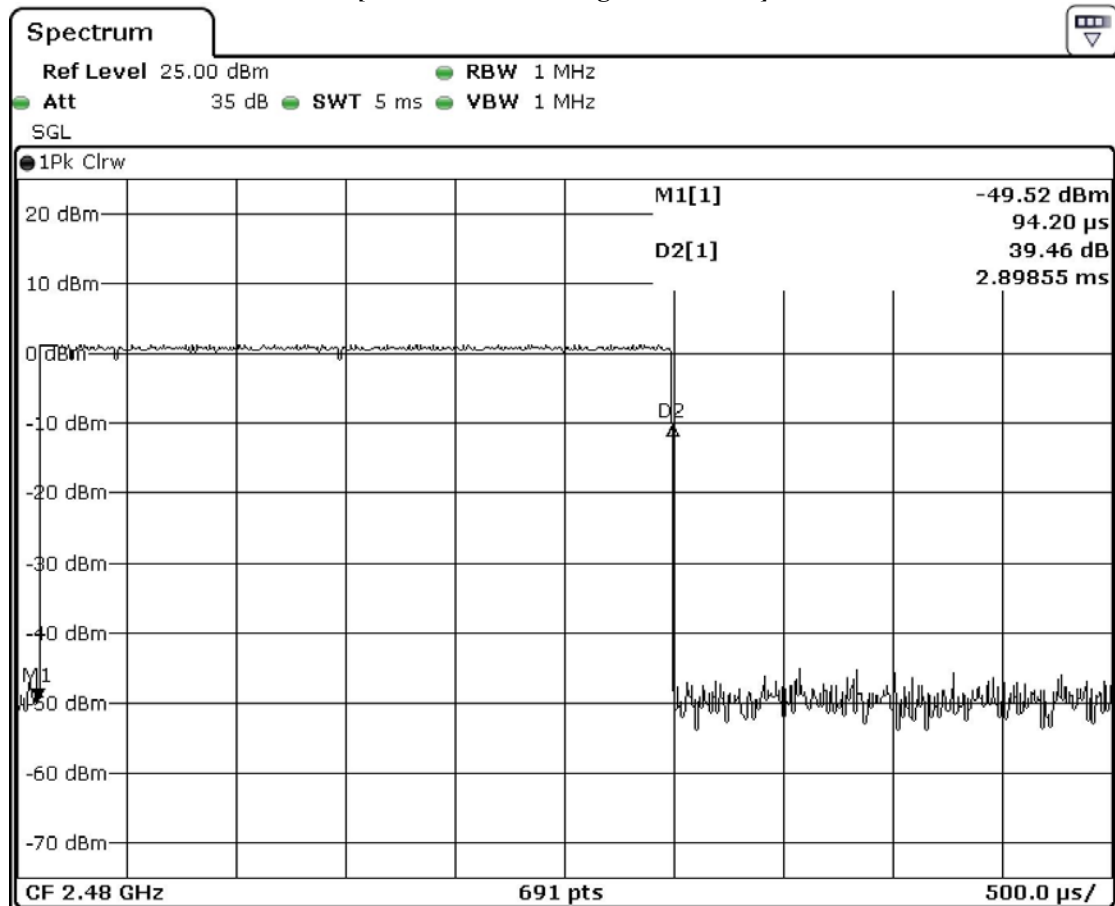
Fig. C [Pulse duration of Highest Channel]
