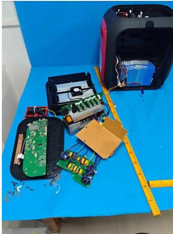
Inner View of the EUT
