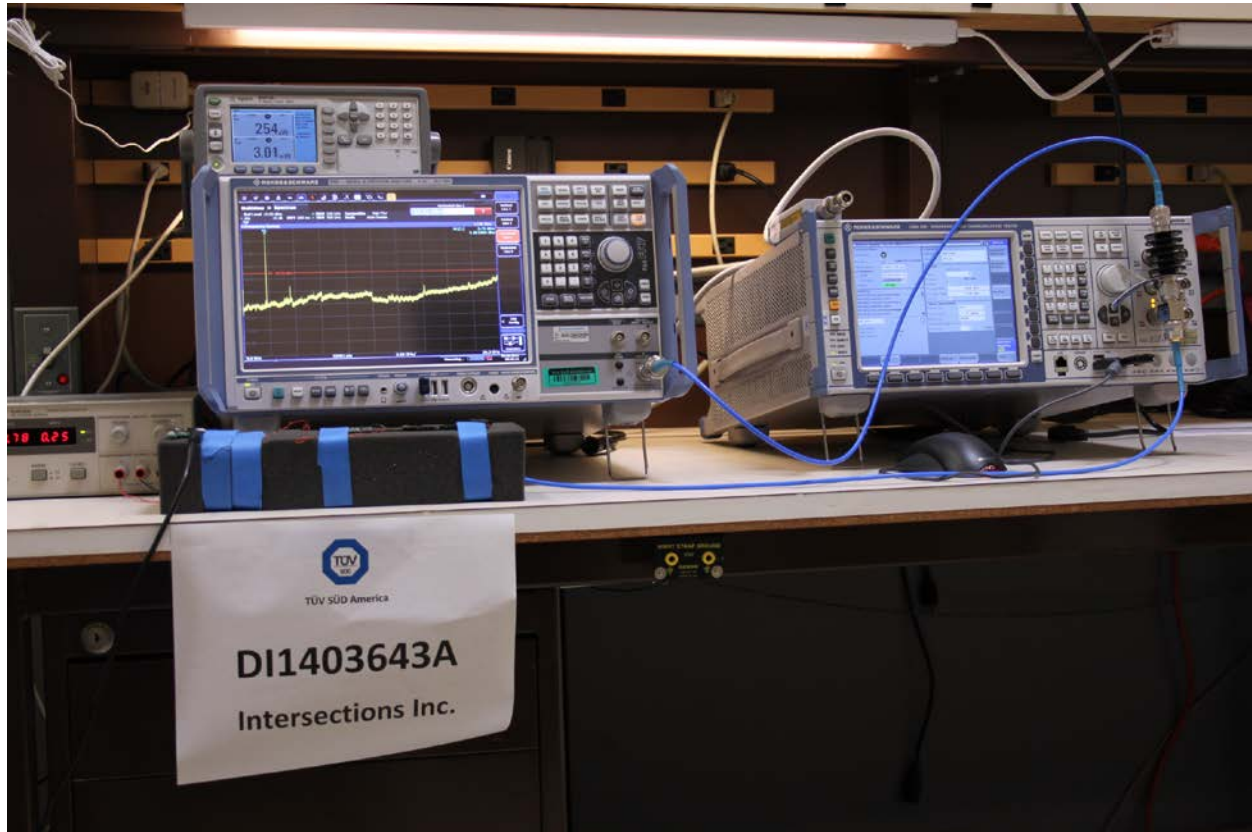
Antenna Conducted Port Test Setup (Open Board Sample)
