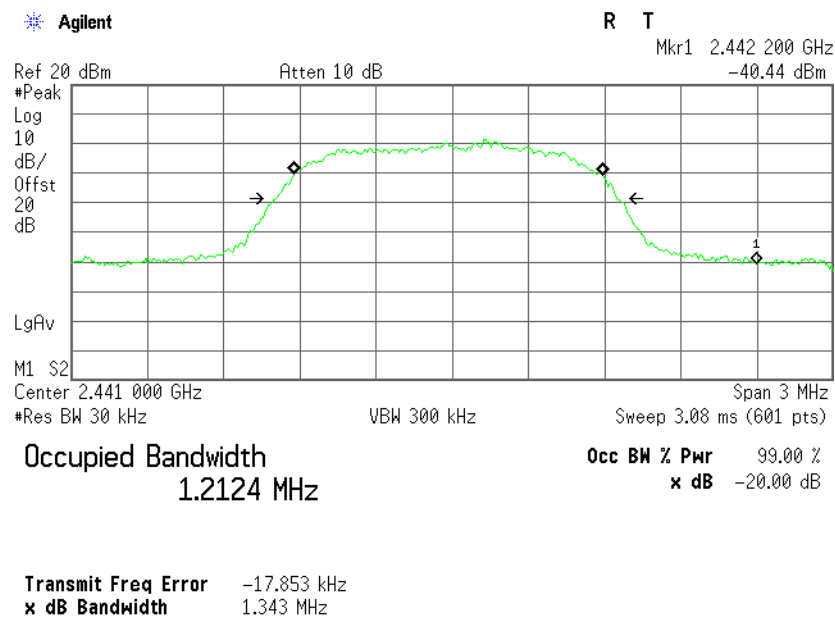
Plot 4.1.5 20dB bandwidth test results, QFSK, channel 39
