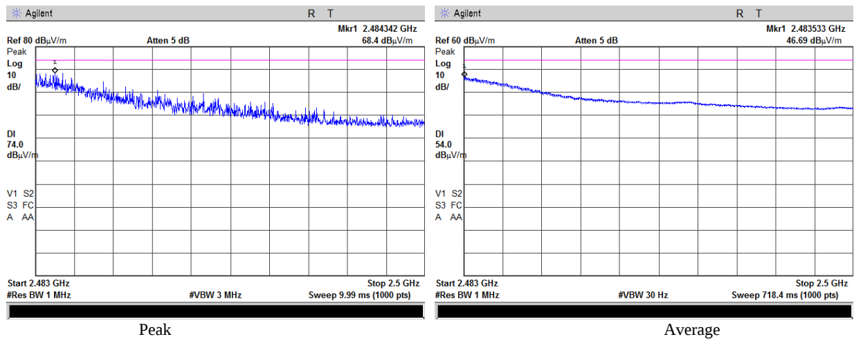
Plot 4.5.4 Radiated Spurious Emission, 802.11n 20MHz, Fc = 2462 MHz, MCS7, 2.4835 – 2.5 GHz range, Vertical
