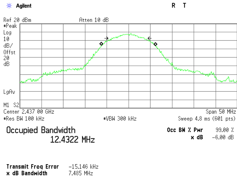
Plot 4.1.2 6dB bandwidth test results, 802.11b Mode, F = 2437 MHz
