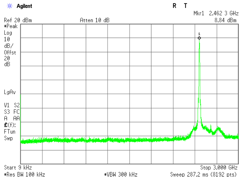
Plot 4.4.8 Conducted Spurious Emissions test results, 802.11b Mode, Fc = 2462 MHz, kHz – 3 GHz range
