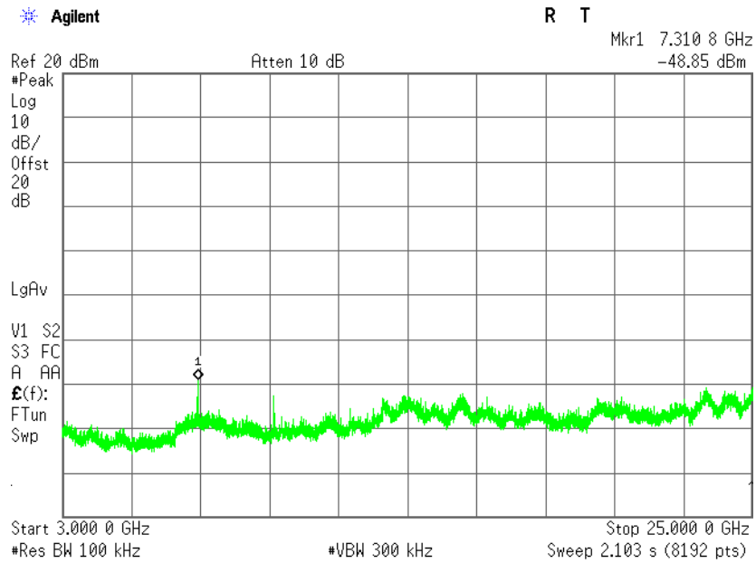
Plot 4.4.6 Conducted Spurious Emissions test results, 802.11b Mode, Fc = 2437 MHz, GHz – 25 GHz range
