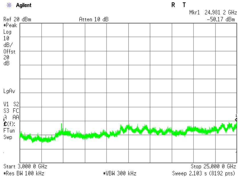
Plot 4.4.12 Conducted Spurious Emissions test results, 802.11g Mode, Fc = 2412 MHz, GHz – 25 GHz range
