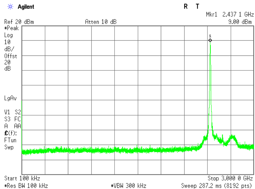
Plot 4.4.5 Conducted Spurious Emissions test results, 802.11b Mode, Fc = 2437 MHz, kHz – 3 GHz range
