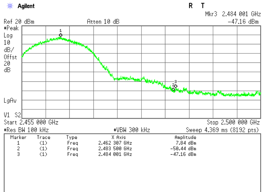
Plot 4.4.29 Band Edge test results, 802.11b Mode, F = 2462 MHz
