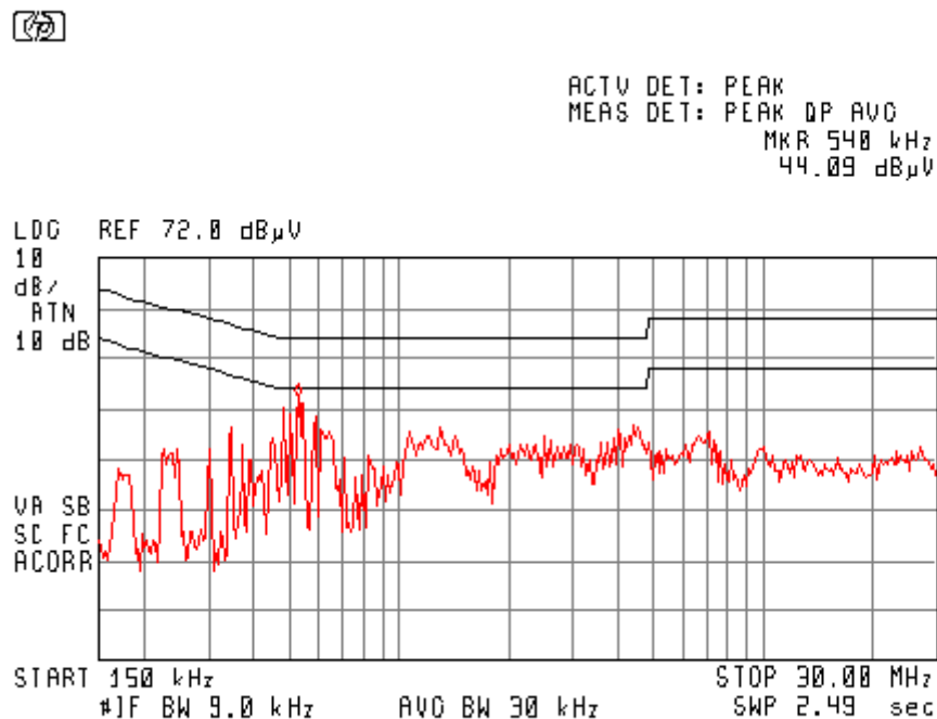
Plot 4.7.2: Neutral Lead
