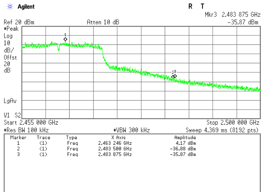
Plot 4.4.31 Band Edge test results, 802.11g Mode, F = 2462 MHz
