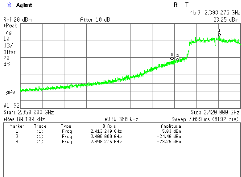
Plot 4.4.30 Band Edge test results, 802.11g Mode, F = 2412 MHz
