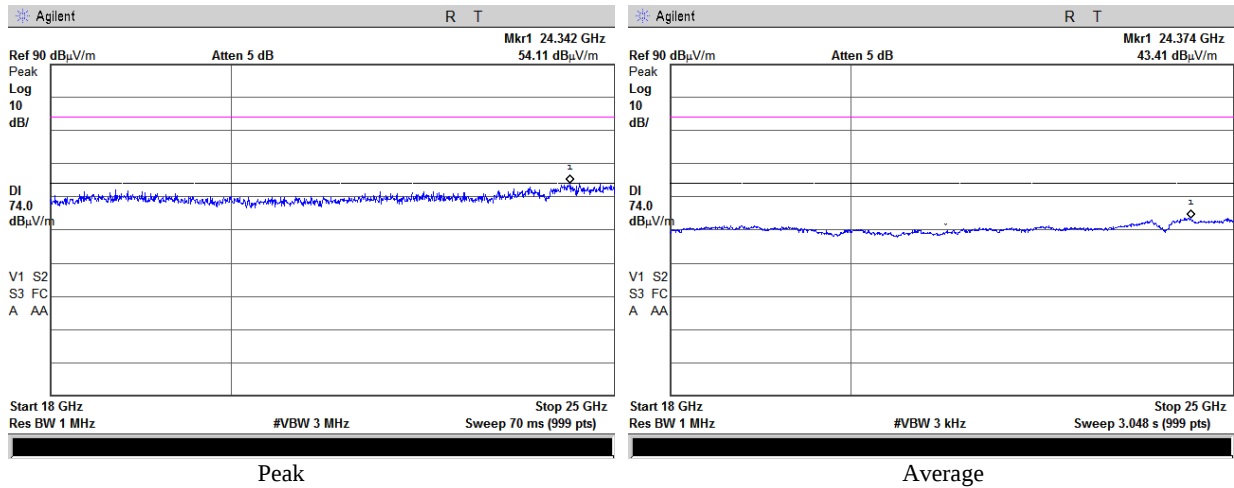
Plot 4.6.17 Radiated Spurious Emission in 18 – 25 GHz range, 802.11n 20MHz, Fc = 2462 MHz, MCS7, Horizontal & Vertical
