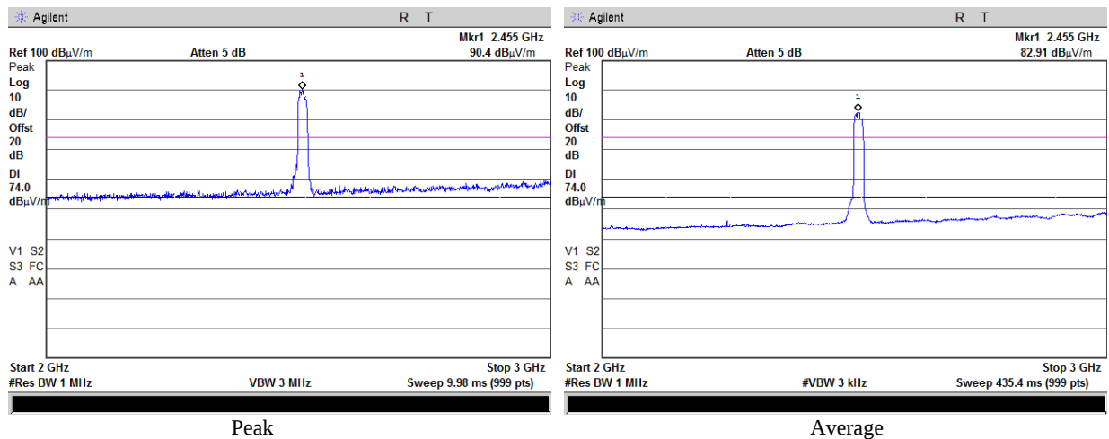
Plot 4.6.14 Radiated Spurious Emission in 2 – 3 GHz range, 802.11n 20MHz, Fc = 2462 MHz, MCS7, Horizontal & Vertical
