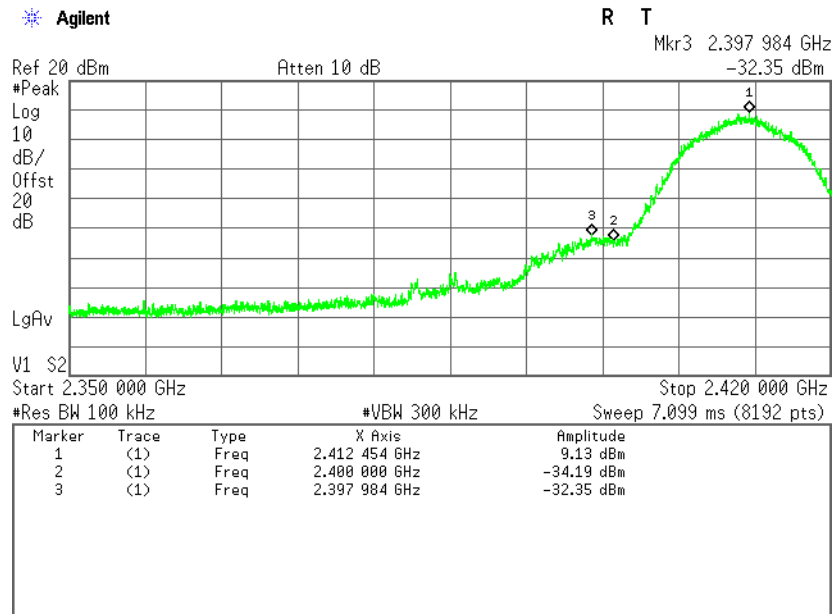
Plot 4.4.28 Band Edge test results, 802.11b Mode, F = 2412 MHz
