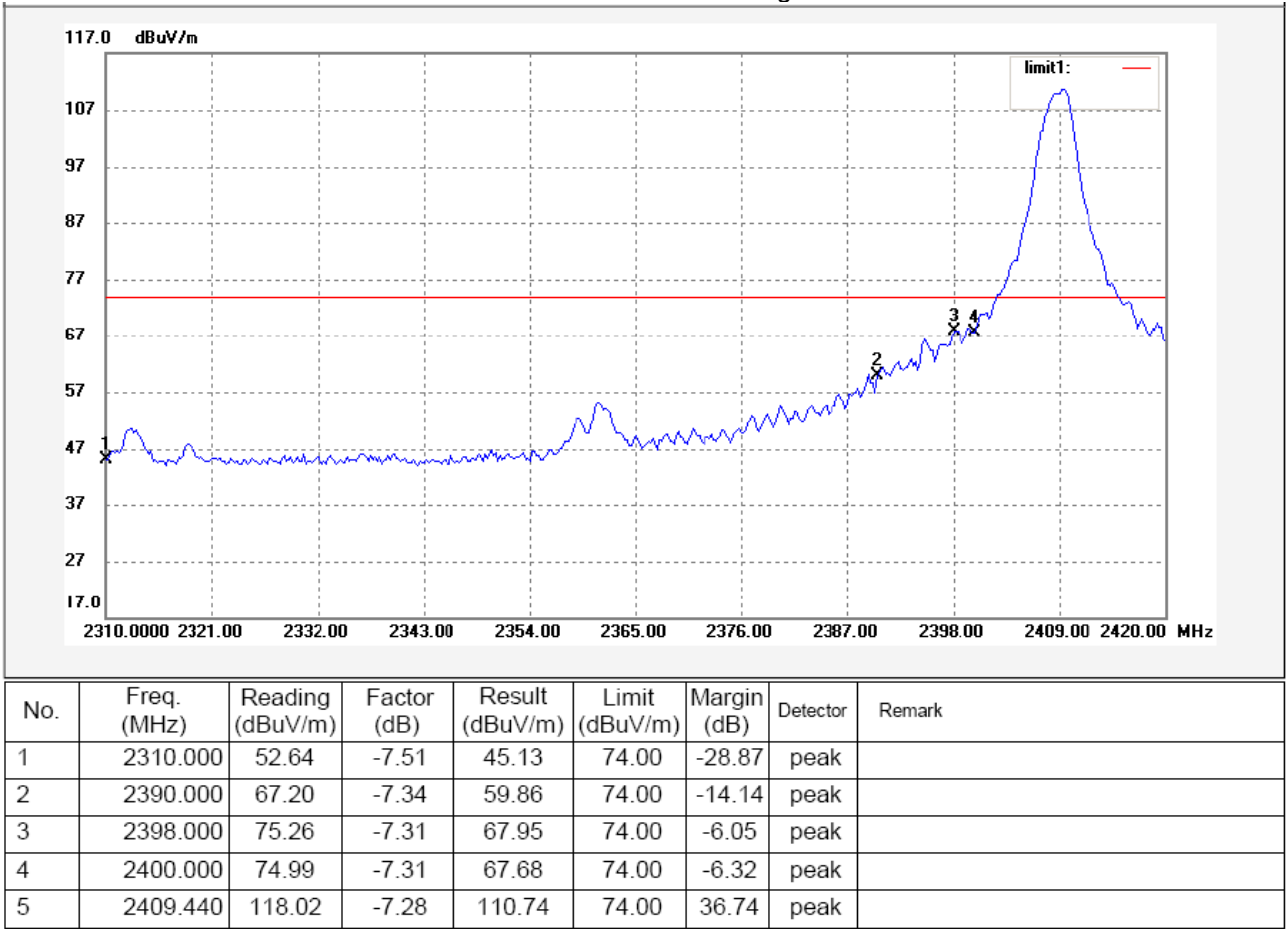
Low Channel – Peak: Transmitting mode
