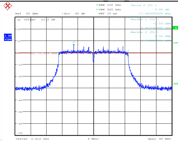
11N20SISO Ant1 2412
