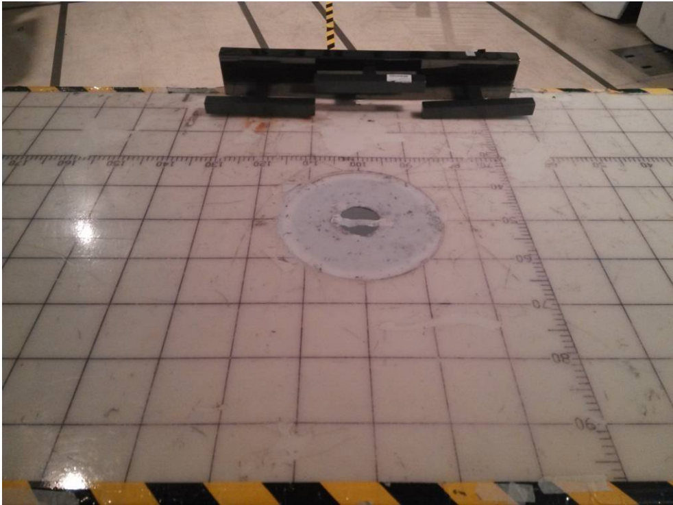
Test Setup Photo –Radiated Emission Below 1GHz
