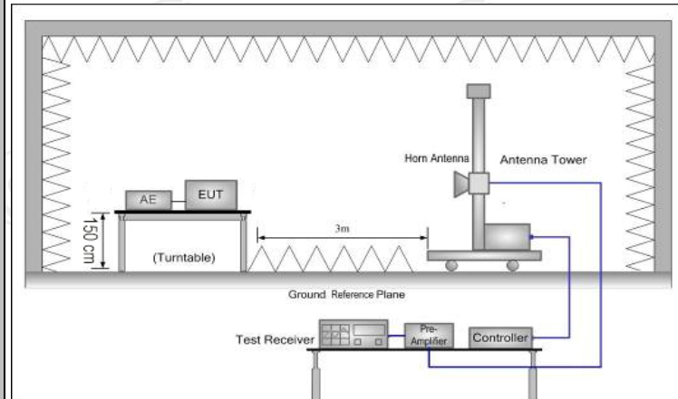
Above 1GHz
