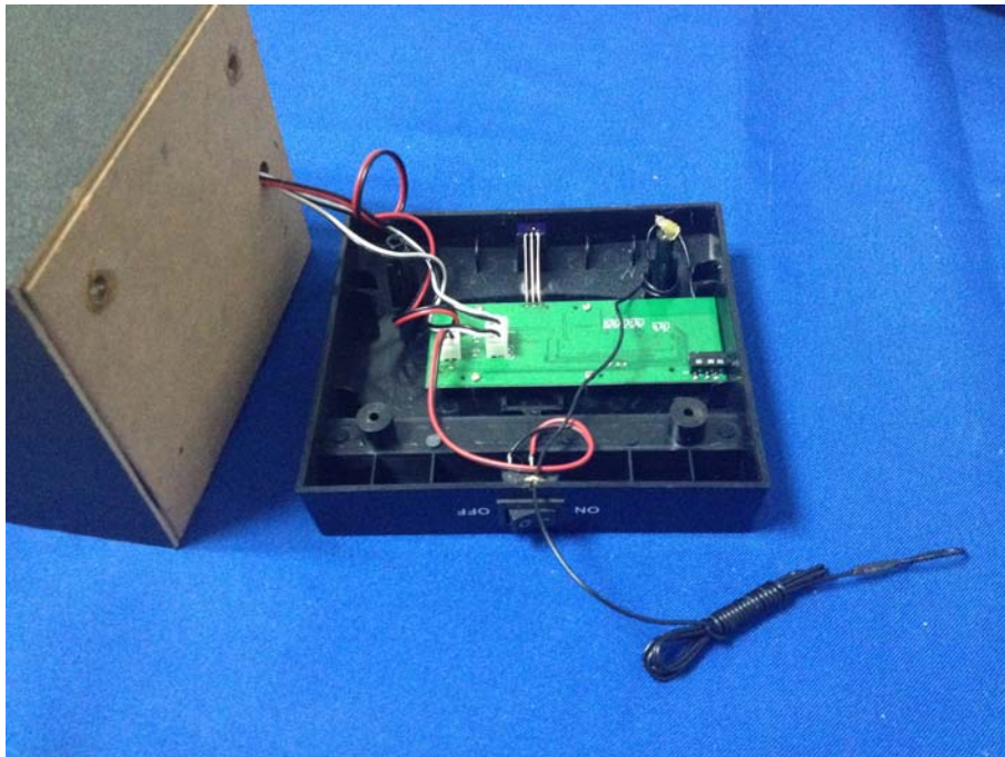
Internal photo (BLUETOOTH SPEAKER Model: PBT3014)
