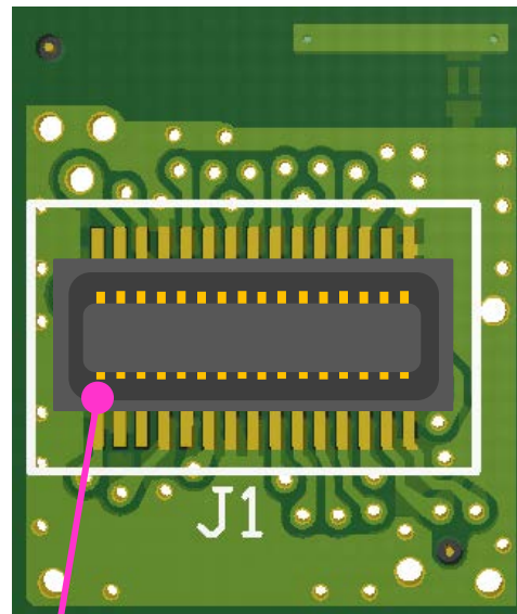
Bottom View
