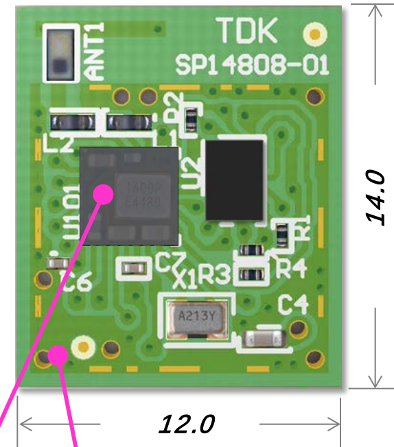
Inside View (Under Metal shield case)
