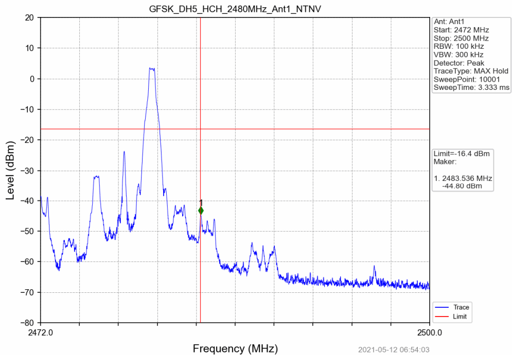
GFSK_DH5_HCH_2480MHz_Ant1_NTNV
