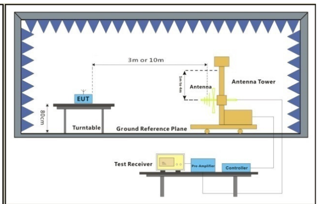
30MHz-1GHz
