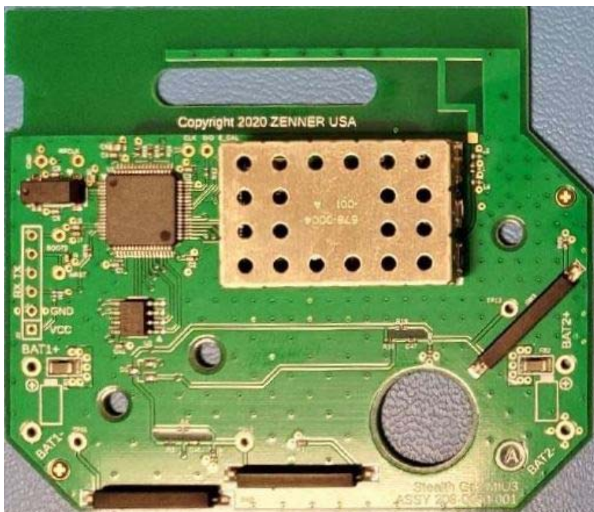
Figure E22.2 – PCB Top
