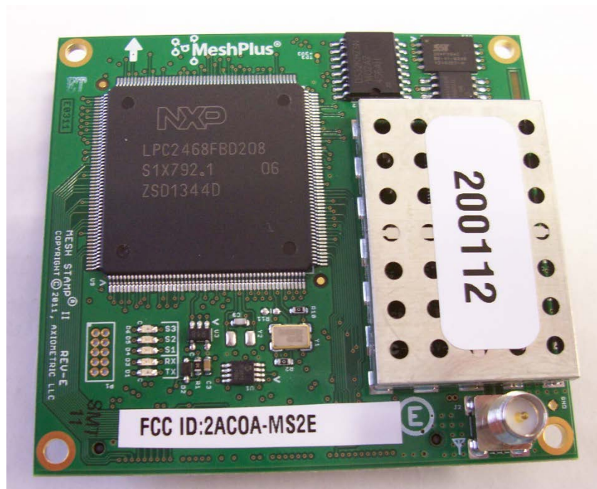
Top View of 2ACOA-MS2E
