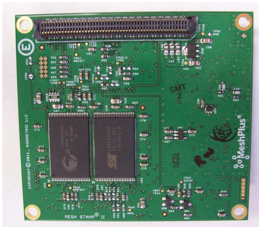
Bottom View of 2ACOA-MS2E
