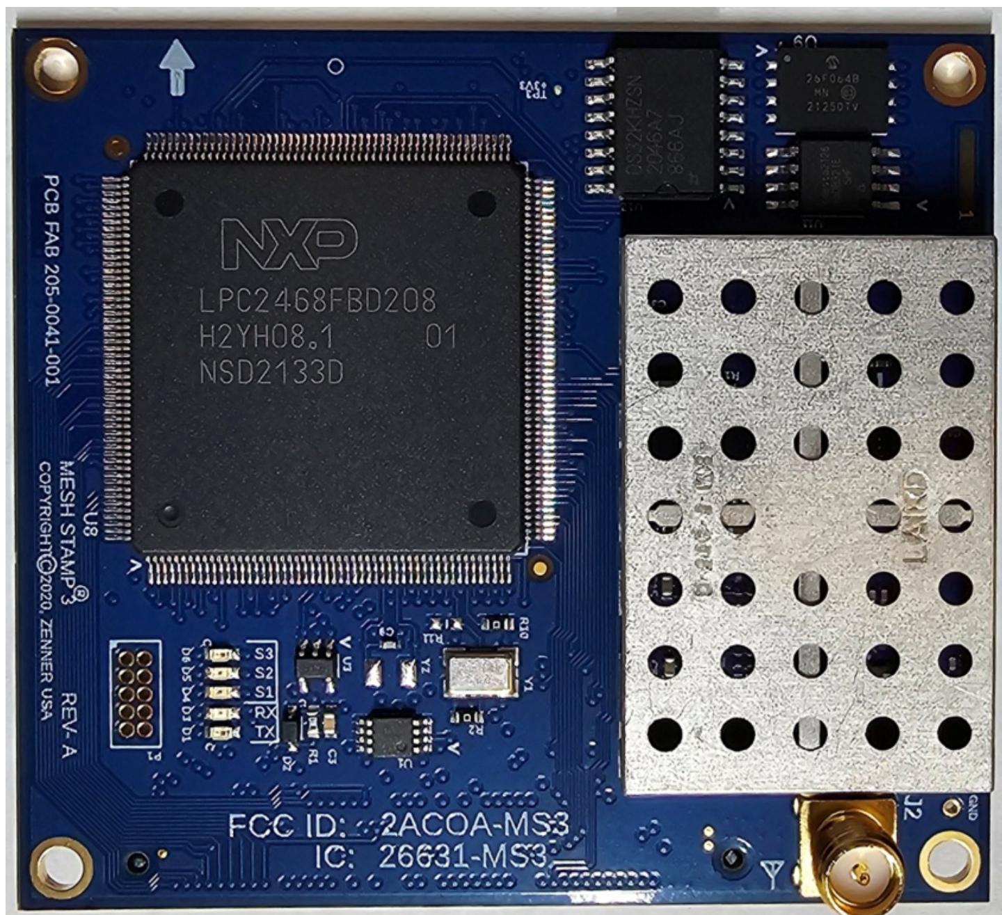
Figure E17.1 – Internal, Top
