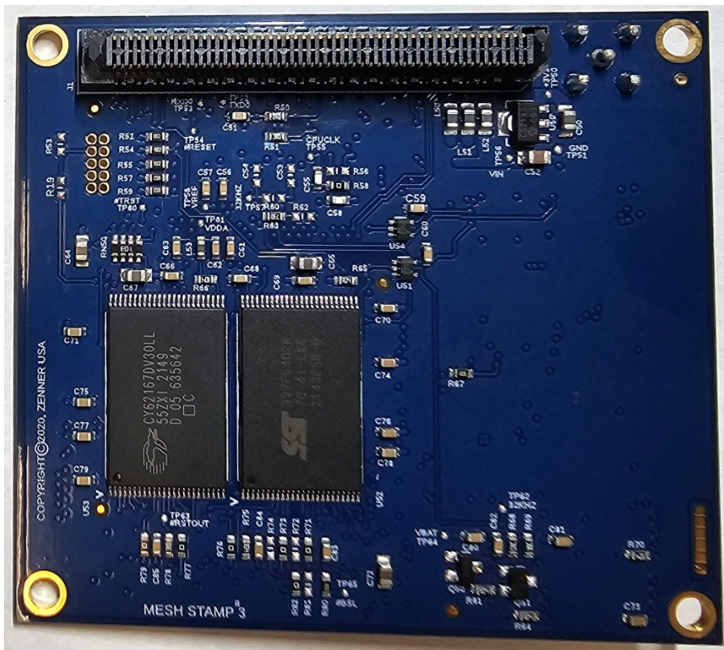
Figure E17.3 – Internal, Bottom
