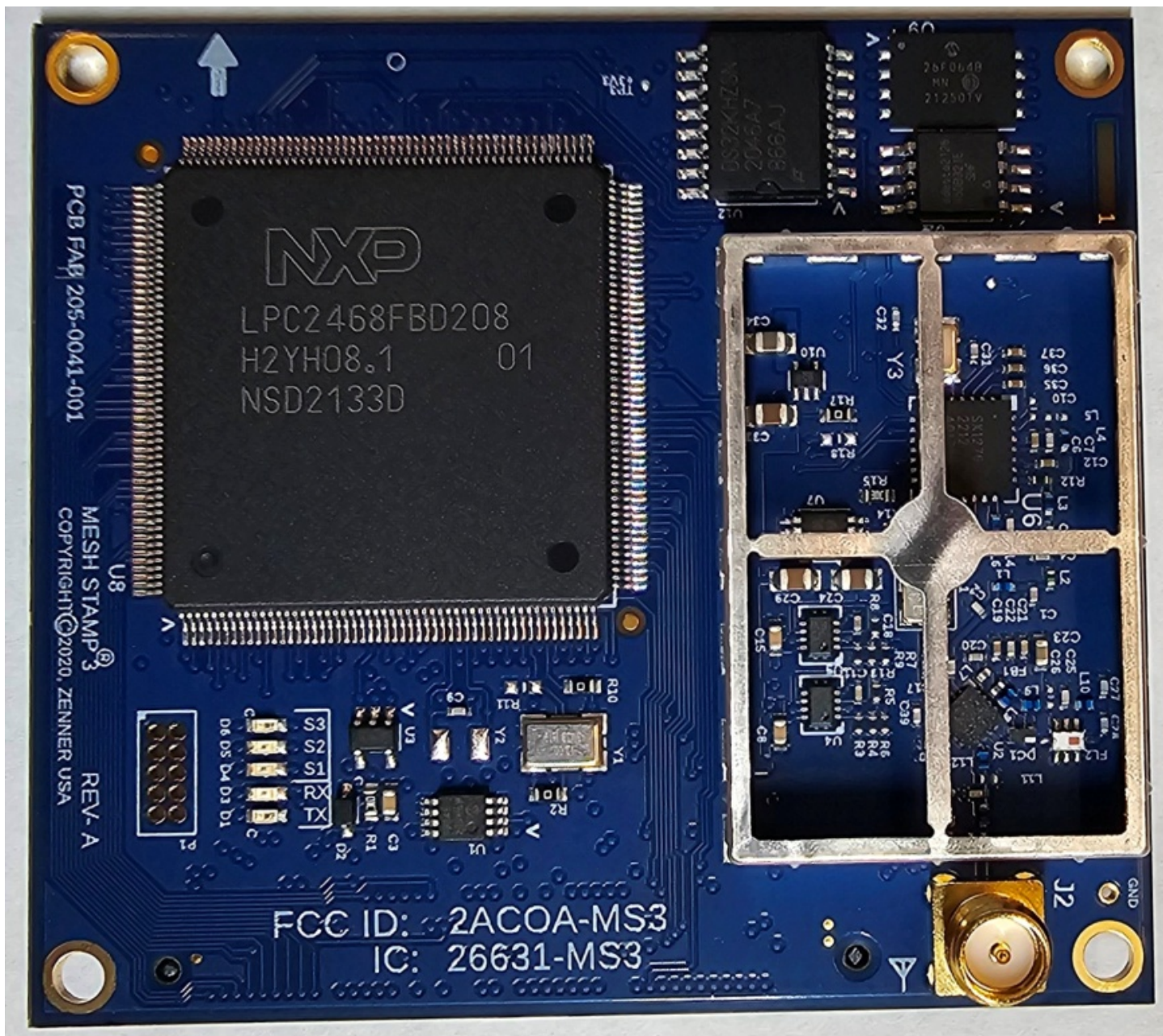
Figure E17.2 – Internal, Top, Shield Removed
