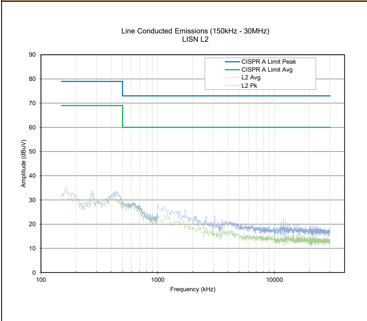
Plot 18.2 – Line Conducted Emissions, L2 Neutral
