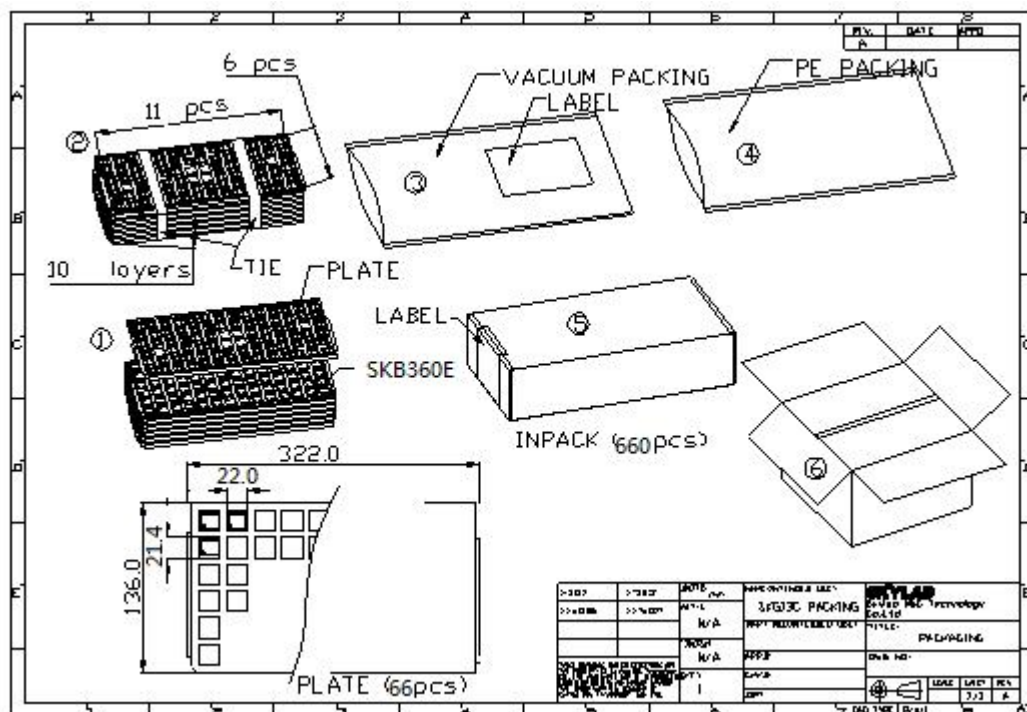
Figure 7: SKB360 Packaging
