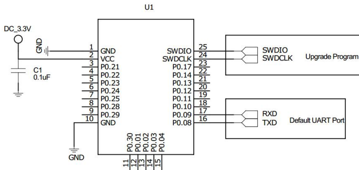
Figure 3: SKB360 schematic
