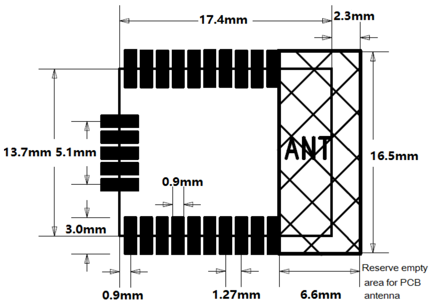
Figure 5: SKB369 Recommended PCB Footprint
