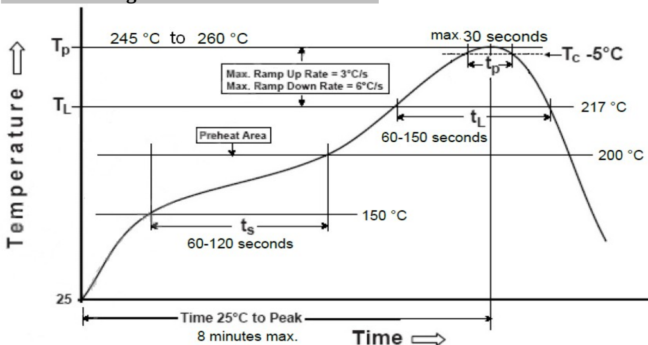
Figure 3: SKW92 Typical Lead-free Soldering Profile
