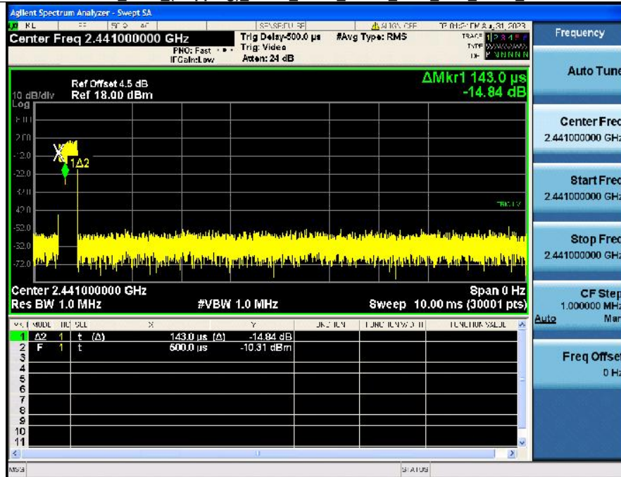
Dwell_Time_(Hopping)_NVNT_ANT1_3-DH1_2441_Accumulated
