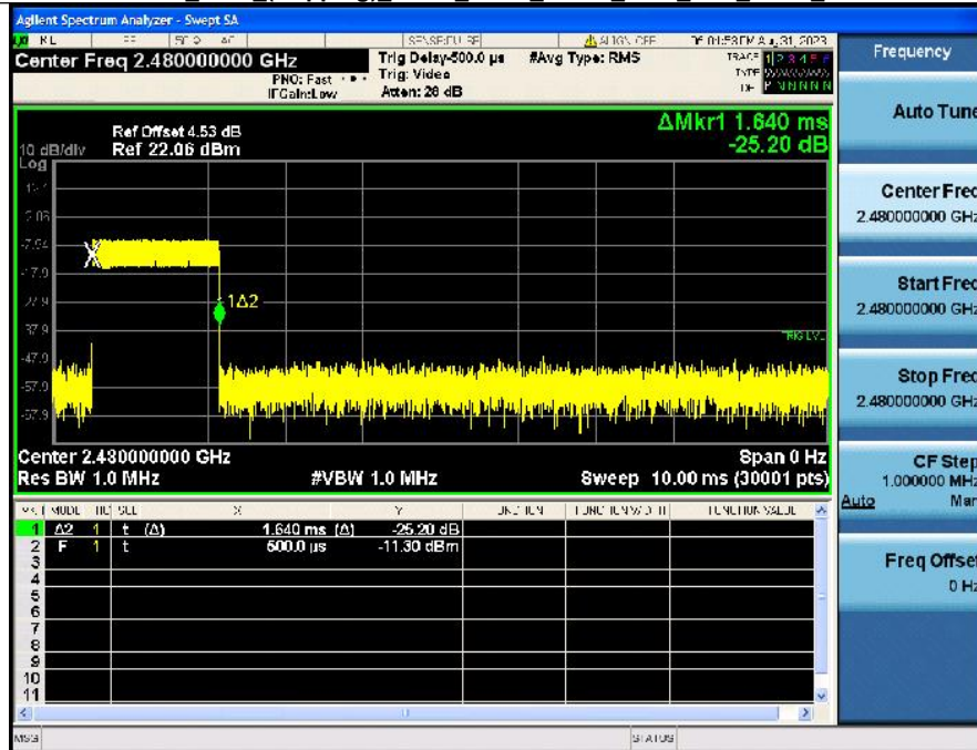
Dwell_Time_(Hopping)_NVNT_ANT1_1-DH3_2480_Accumulated
