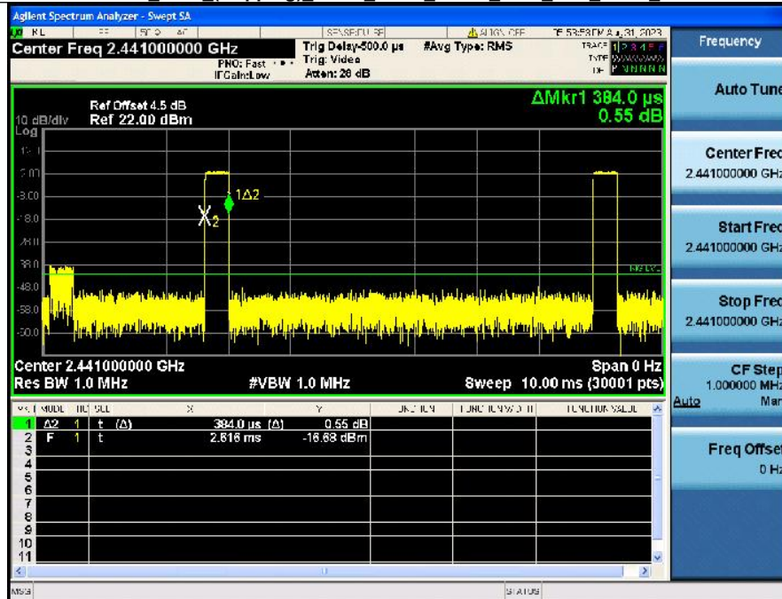
Dwell_Time_(Hopping)_NVNT_ANT1_1-DH1_2441_Accumulated
