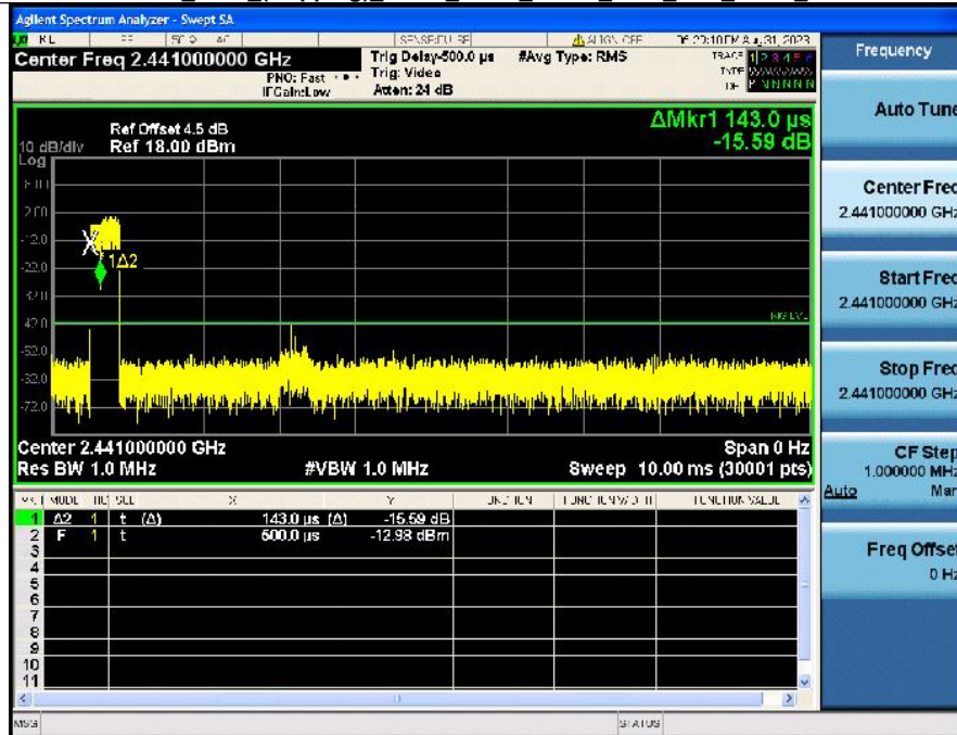
Dwell_Time_(Hopping)_NVNT_ANT1_2-DH1_2441_Accumulated
