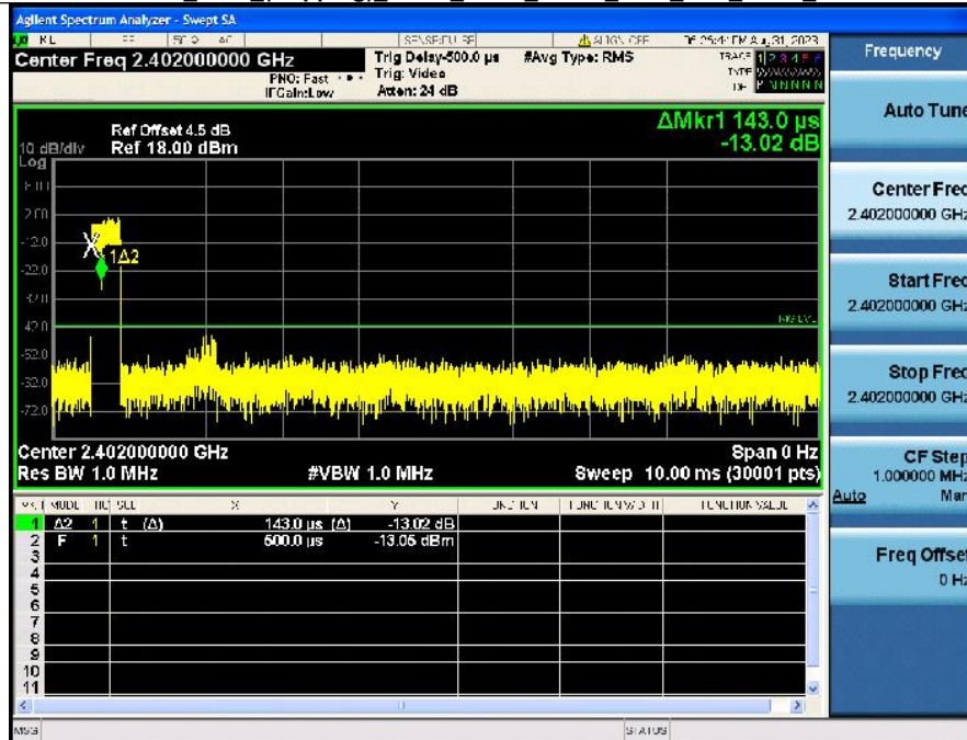
Dwell_Time_(Hopping)_NVNT_ANT1_2-DH1_2402_Accumulated
