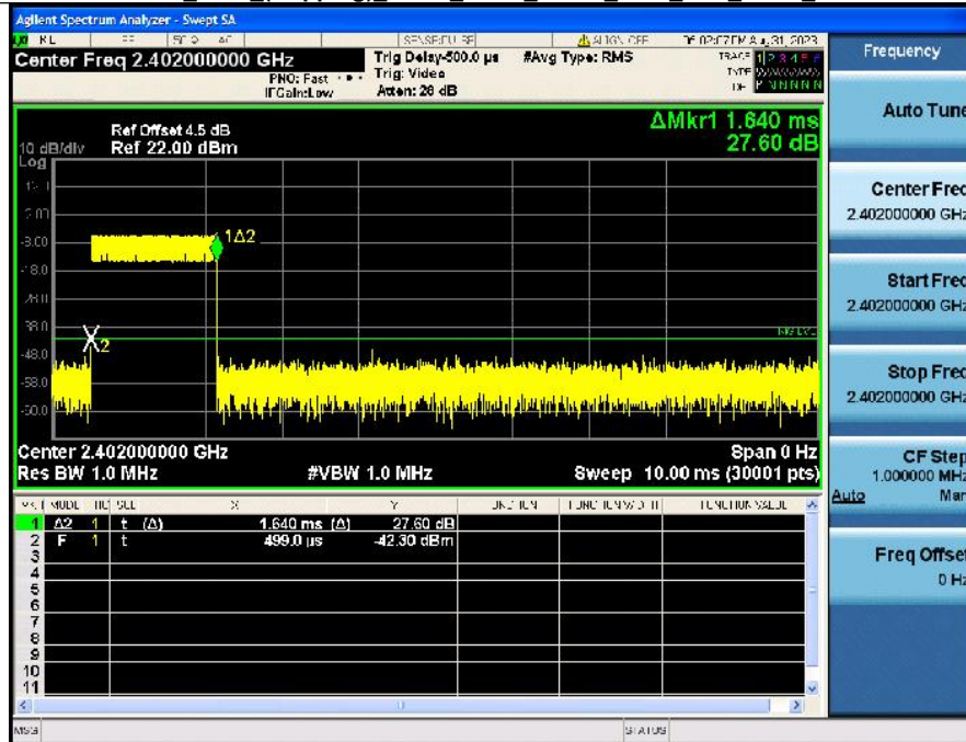
Dwell_Time_(Hopping)_NVNT_ANT1_1-DH3_2402_Accumulated
