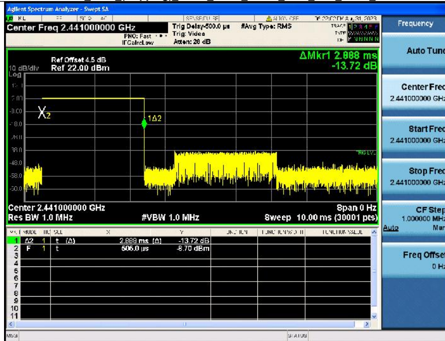
Dwell_Time_(Hopping)_NVNT_ANT1_1-DH5_2441_Accumulated
