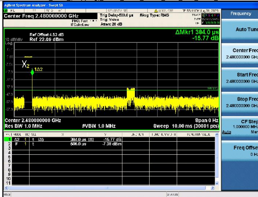
Dwell_Time_(Hopping)_NVNT_ANT1_1-DH1_2480_Accumulated
