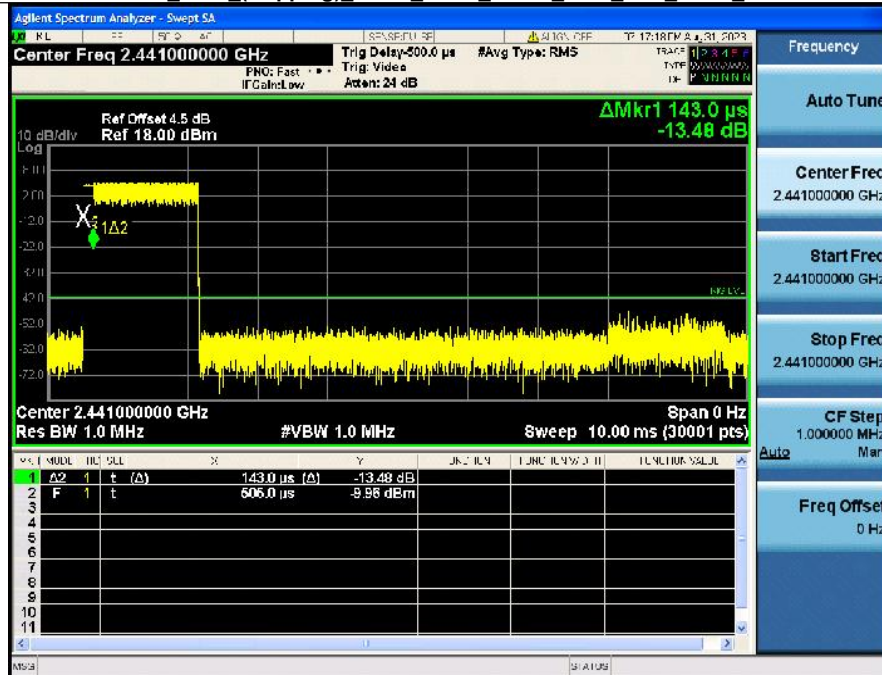
Dwell_Time_(Hopping)_NVNT_ANT1_3-DH3_2441_Accumulated
