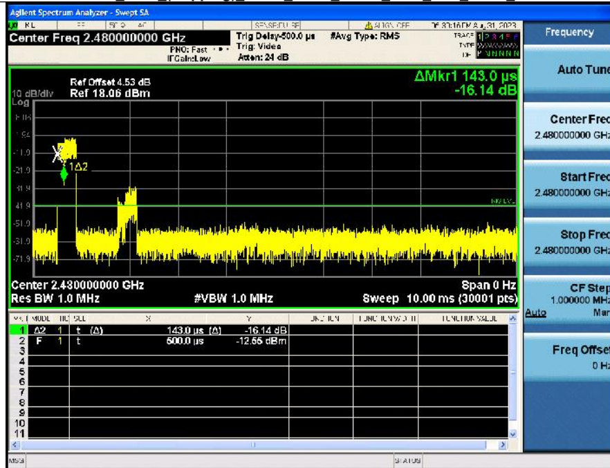
Dwell_Time_(Hopping)_NVNT_ANT1_2-DH1_2480_Accumulated
