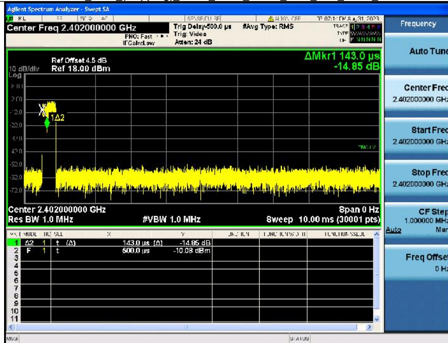
Dwell_Time_(Hopping)_NVNT_ANT1_3-DH1_2402_Accumulated
