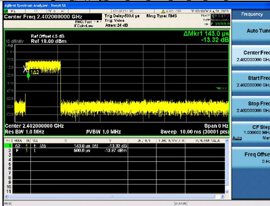
Dwell_Time_(Hopping)_NVNT_ANT1_3-DH3_2402_Accumulated
