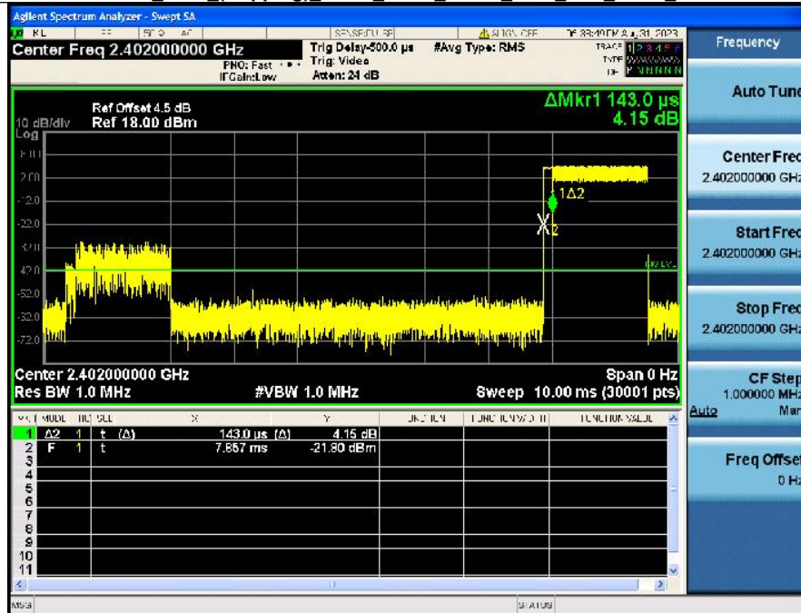
Dwell_Time_(Hopping)_NVNT_ANT1_2-DH3_2402_Accumulated
