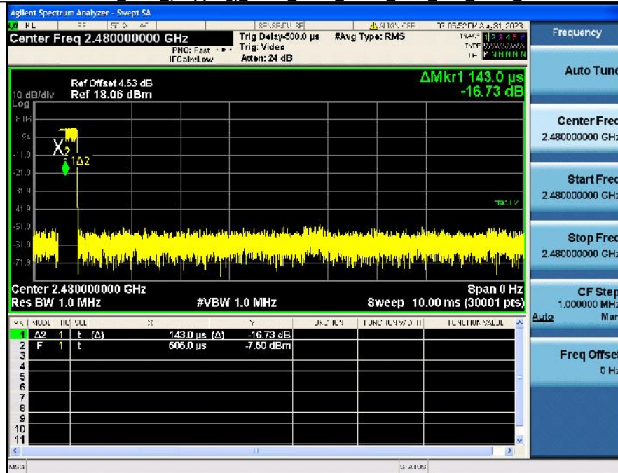
Dwell_Time_(Hopping)_NVNT_ANT1_3-DH1_2480_Accumulated
