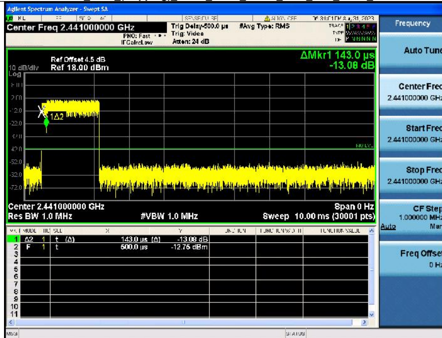
Dwell_Time_(Hopping)_NVNT_ANT1_2-DH3_2441_Accumulated
