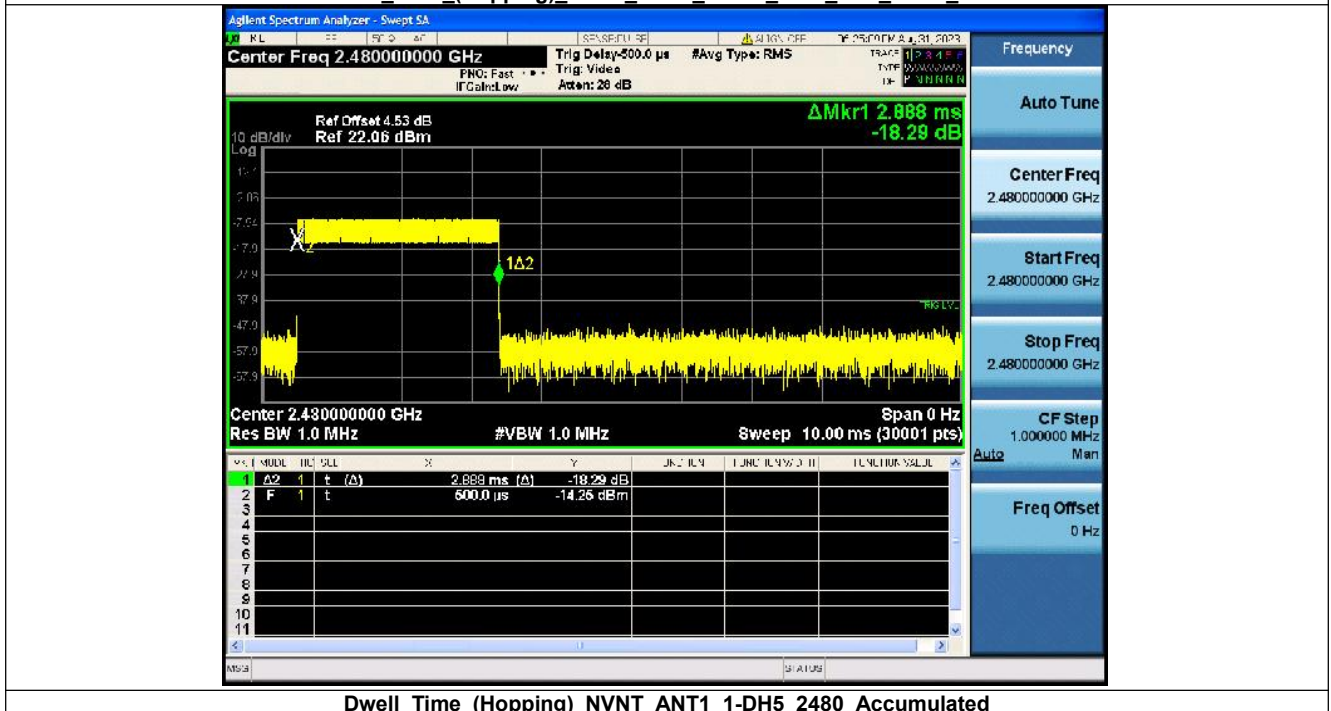
Dwell_Time_(Hopping)_NVNT_ANT1_1-DH5_2480_Accumulated
