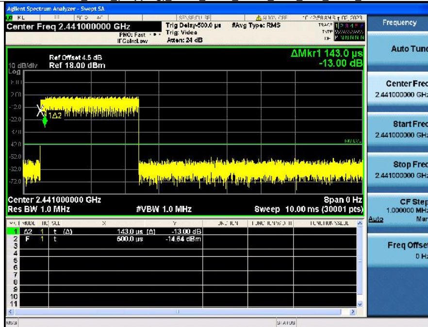
Dwell_Time_(Hopping)_NVNT_ANT1_3-DH5_2441_Accumulated
