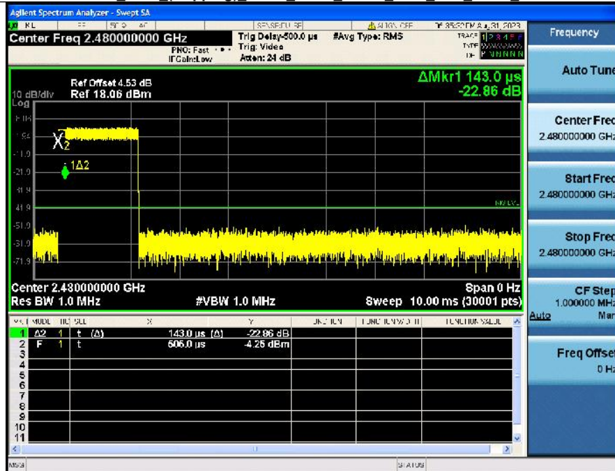
Dwell_Time_(Hopping)_NVNT_ANT1_2-DH3_2480_Accumulated
