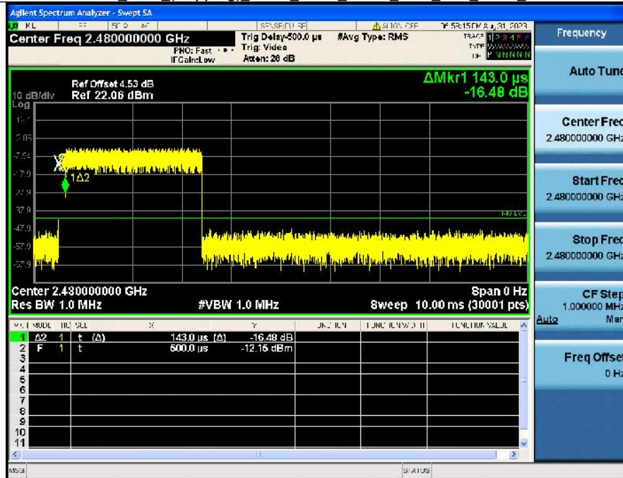
Dwell_Time_(Hopping)_NVNT_ANT1_2-DH5_2480_Accumulated
