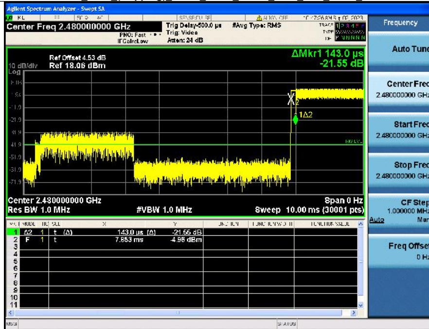
Dwell Time (Hopping) NVNT_ANT1_3-DH5_2480_Accumulated
