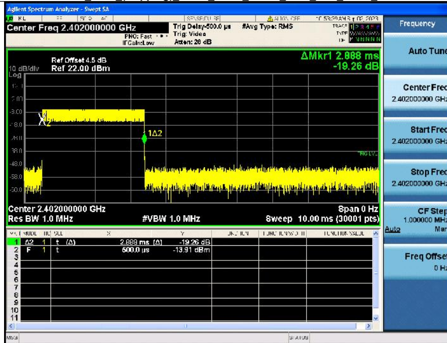
Dwell_Time_(Hopping)_NVNT_ANT1_1-DH5_2402_Accumulated
