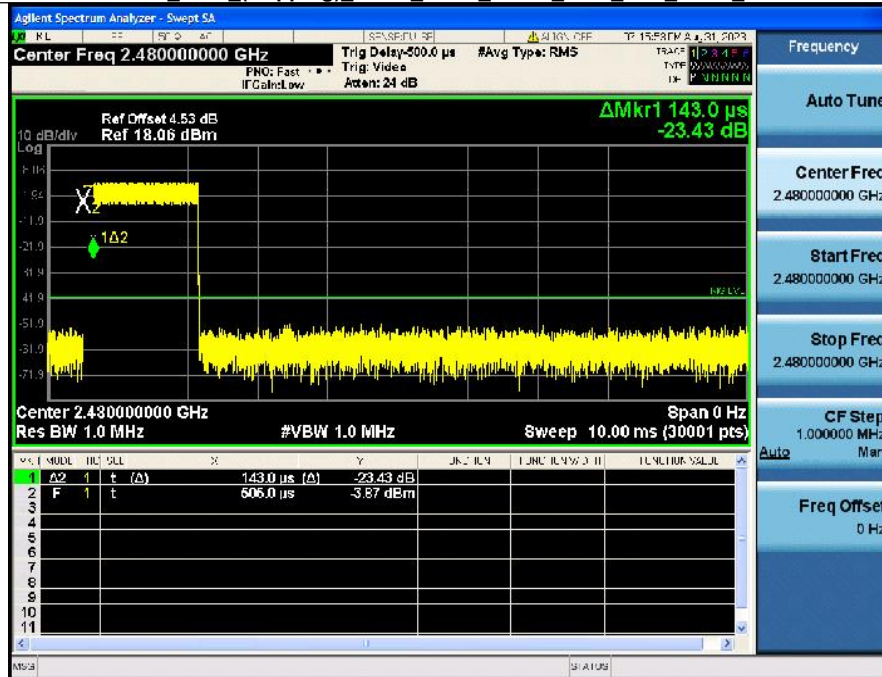
Dwell_Time_(Hopping)_NVNT_ANT1_3-DH3_2480_Accumulated
