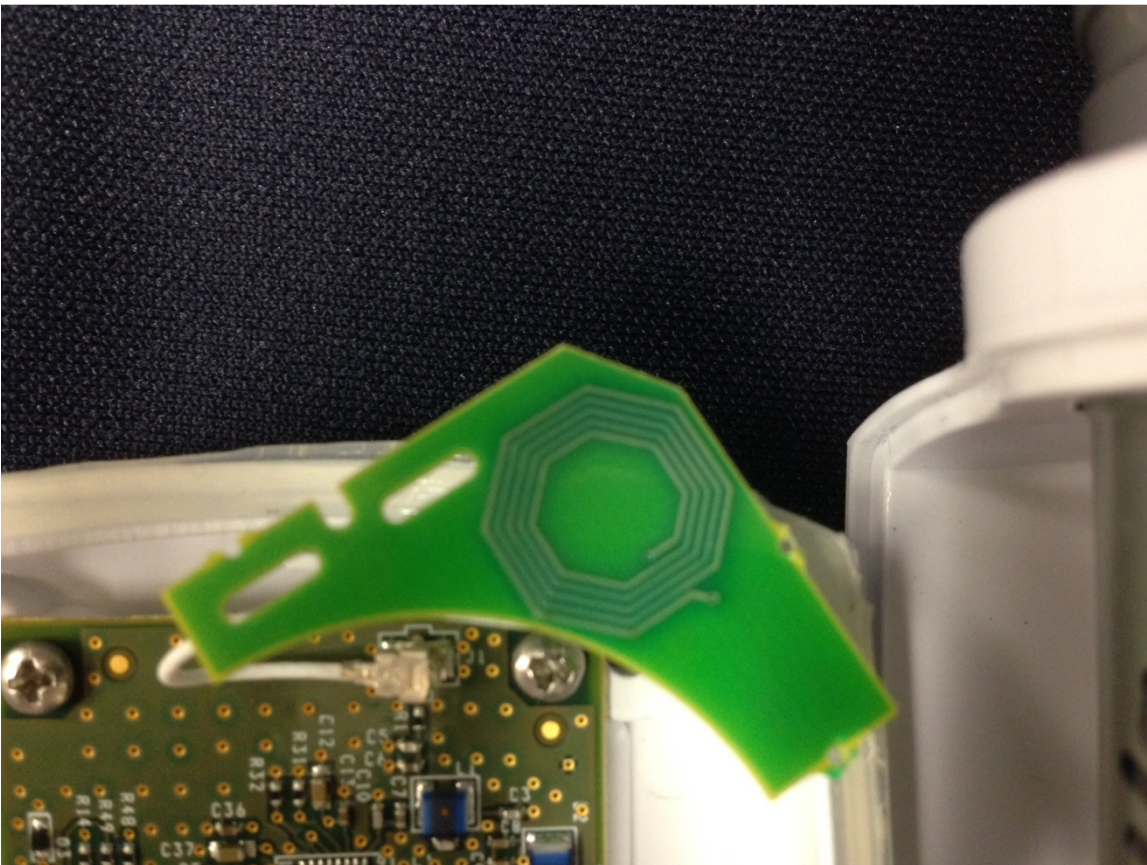
Figure 2: Back of RF Board
