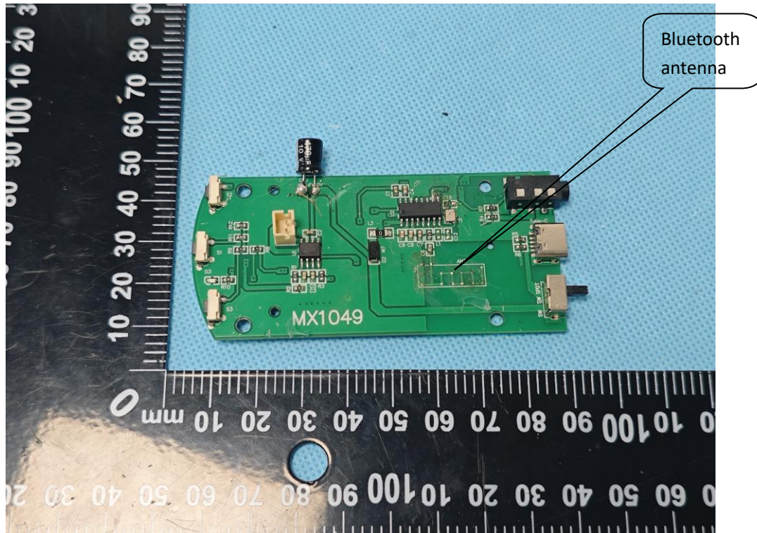
Internal Photo 5
