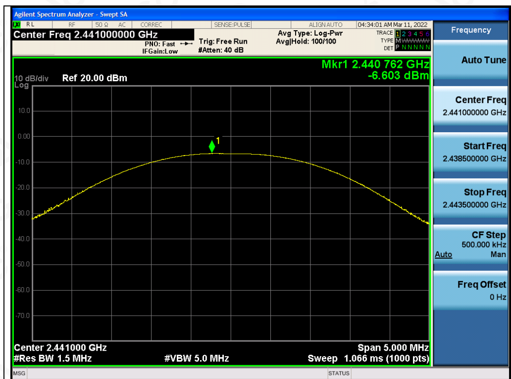
Test Graph EDR ANT1 2441 3Mbps Peak Power
