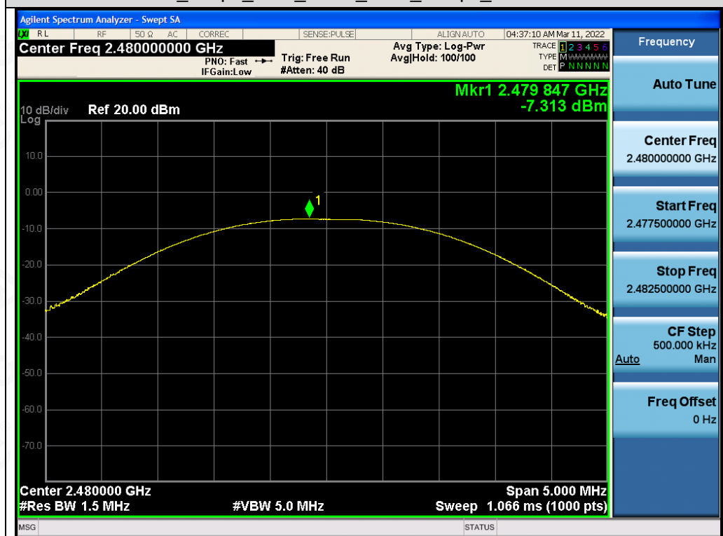
Test Graph EDR ANT1 2480 3Mbps Peak Power
