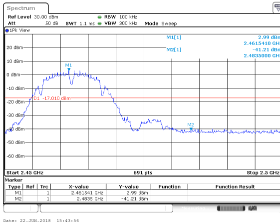
802.11b: Band Edge-High Channel
