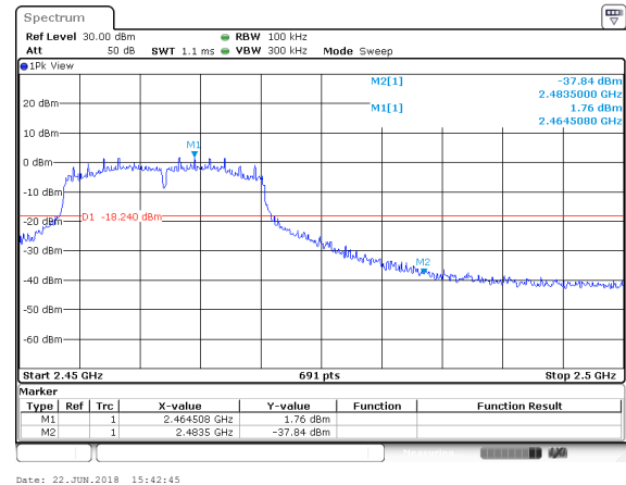
802.11g: Band Edge-High Channel
