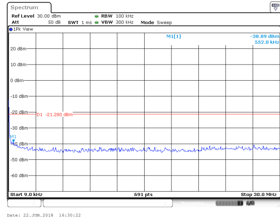
802.11n40 on channel 03
