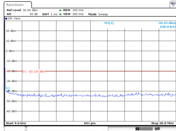
802.11 n40 on channel 9
