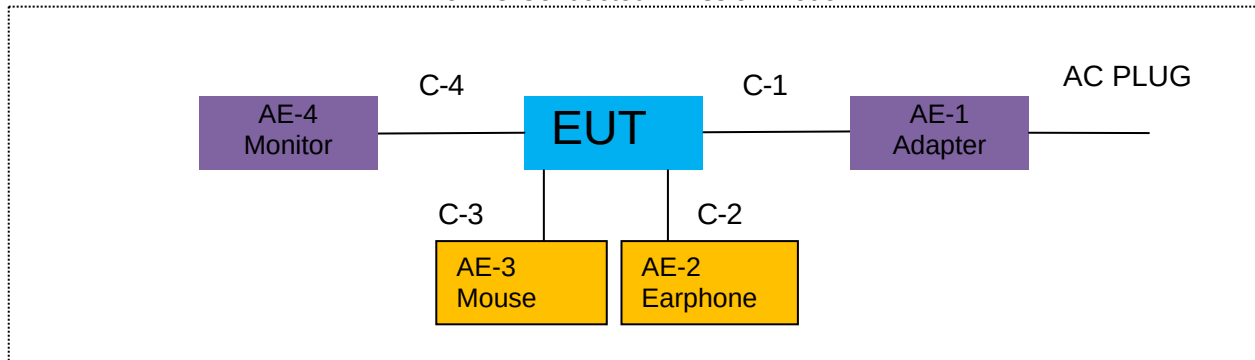
For AC Conducted Emission Mode
