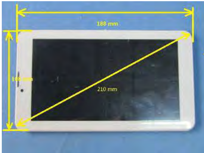
Overall Dimensions
